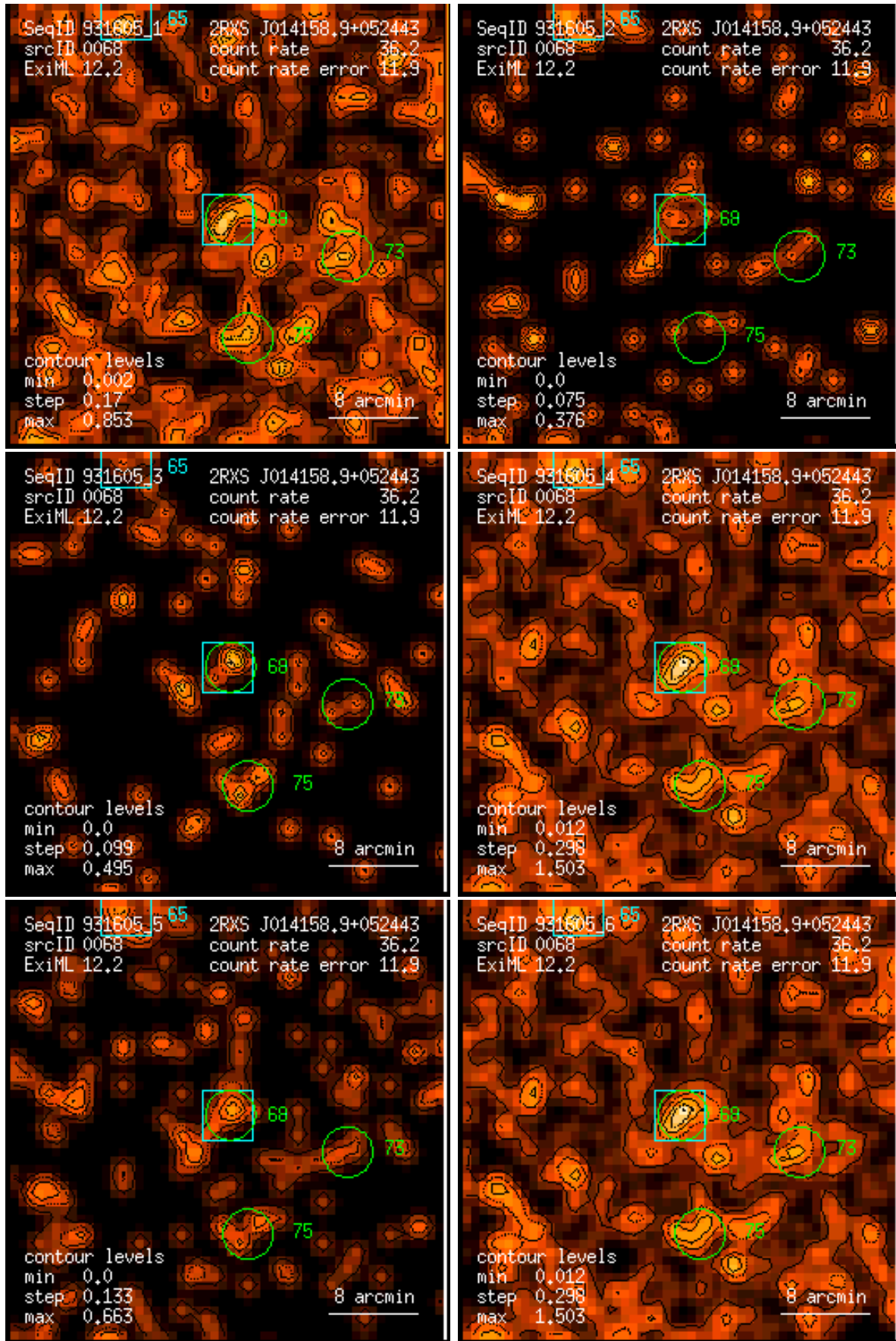
Figure 68: RASS 931605: detection 0068: band rate images, Gaussian filter: (1) PSPC channels 11 – 41, (2) 52 – 90, (3) 91 – 201, (4) 11 – 235, (5) 52 – 201, (6) 11 – 201. Broad band rates in counts/ks. Band rate contour levels in counts/ks/arcmin 2 .
