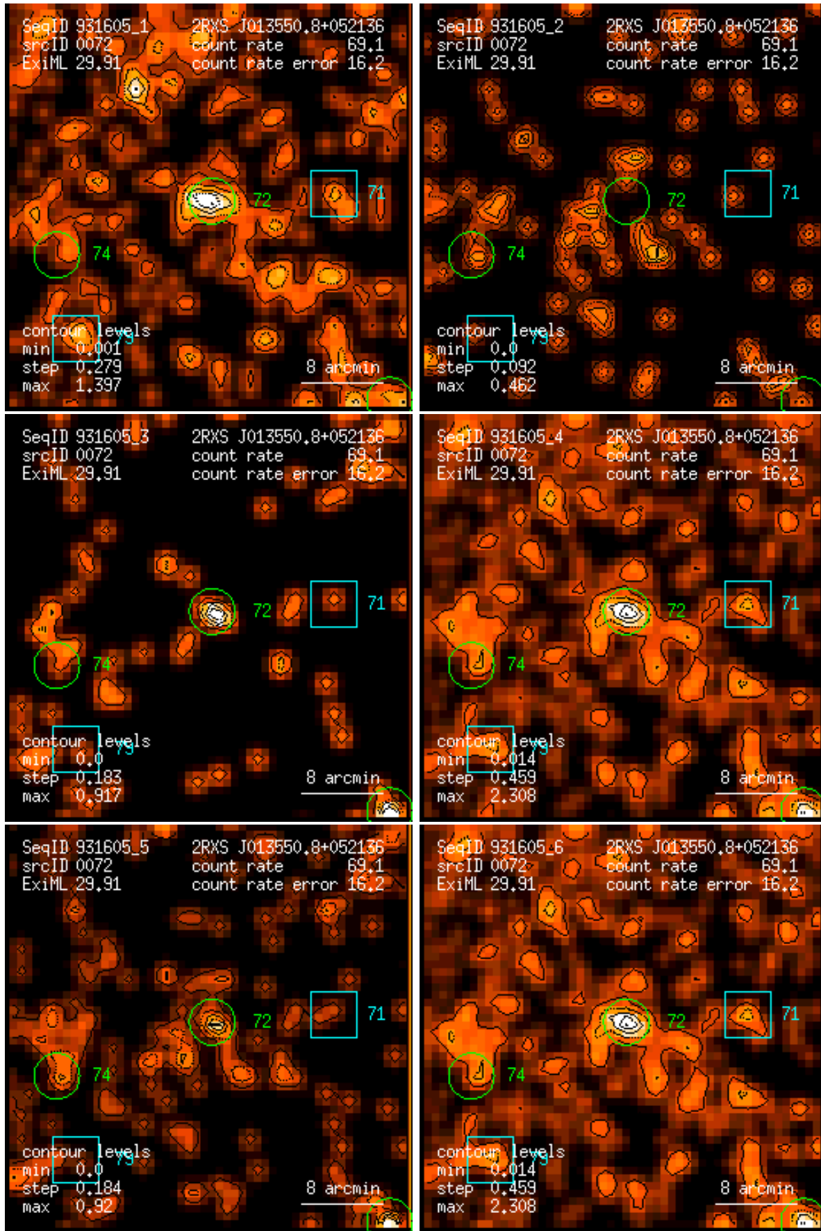
Figure 72: RASS 931605: detection 0072: band rate images, Gaussian filter: (1) PSPC channels 11 – 41, (2) 52 – 90, (3) 91 – 201, (4) 11 – 235, (5) 52 – 201, (6) 11 – 201. Broad band rates in counts/ks. Band rate contour levels in counts/ks/arcmin 2 .
