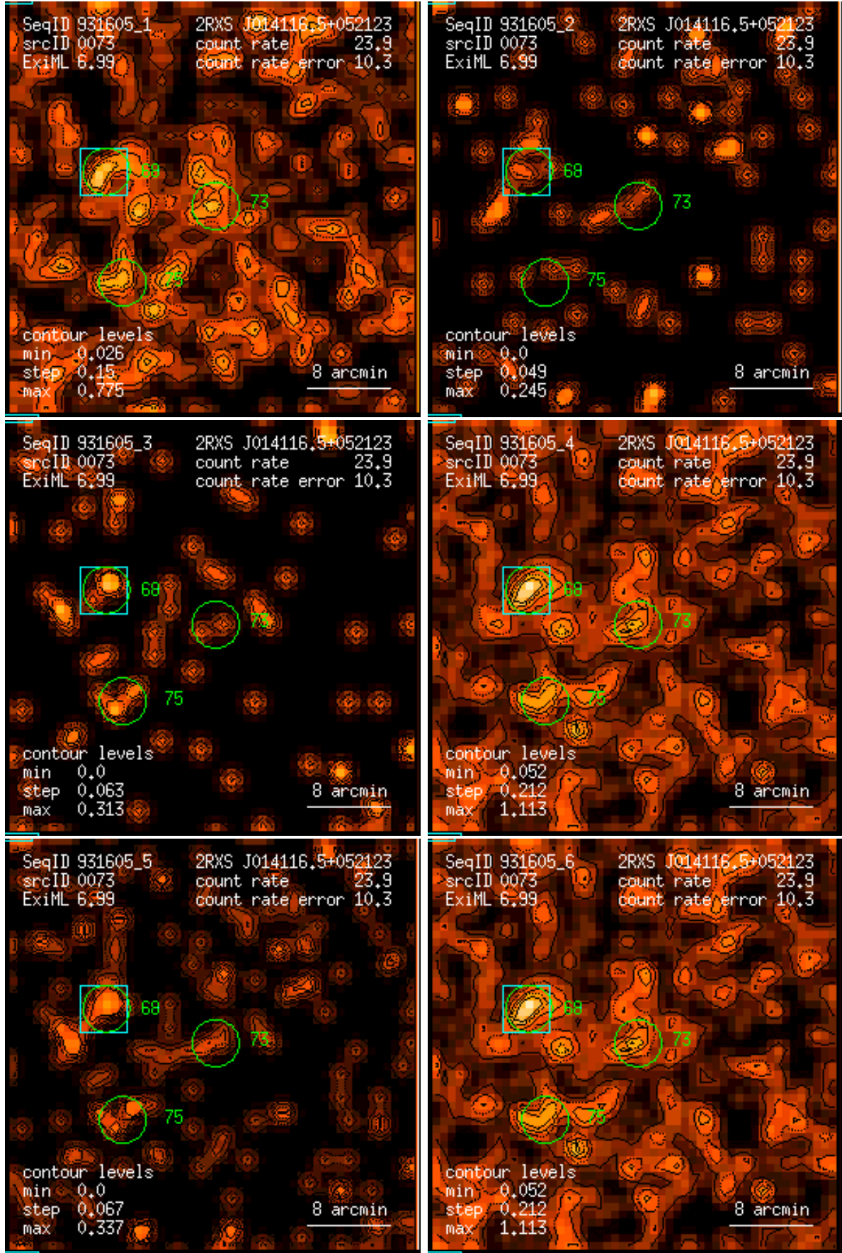
Figure 73: RASS 931605: detection 0073: band rate images, Gaussian filter: (1) PSPC channels 11 – 41, (2) 52 – 90, (3) 91 – 201, (4) 11 – 235, (5) 52 – 201, (6) 11 – 201. Broad band rates in counts/ks. Band rate contour levels in counts/ks/arcmin 2 .
