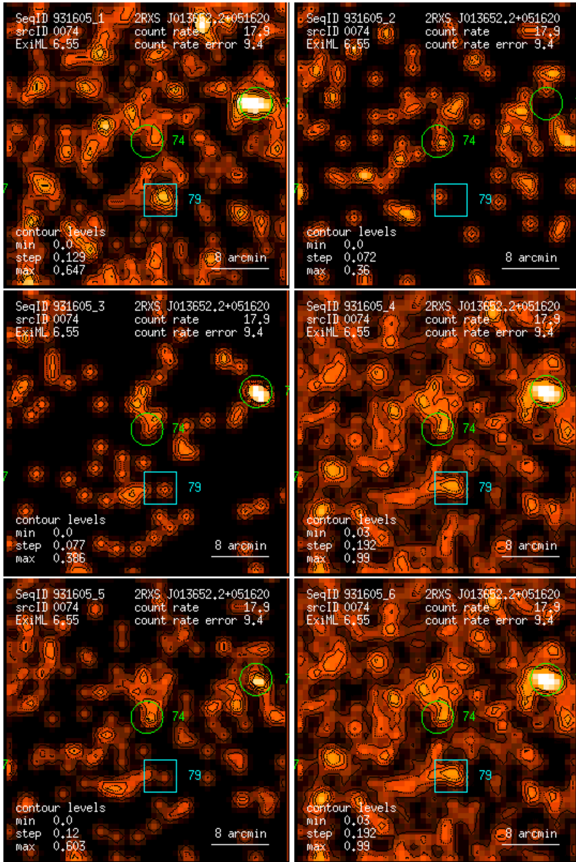
Figure 74: RASS 931605: detection 0074: band rate images, Gaussian filter: (1) PSPC channels 11 – 41, (2) 52 – 90, (3) 91 – 201, (4) 11 – 235, (5) 52 – 201, (6) 11 – 201. Broad band rates in counts/ks. Band rate contour levels in counts/ks/arcmin 2 .
