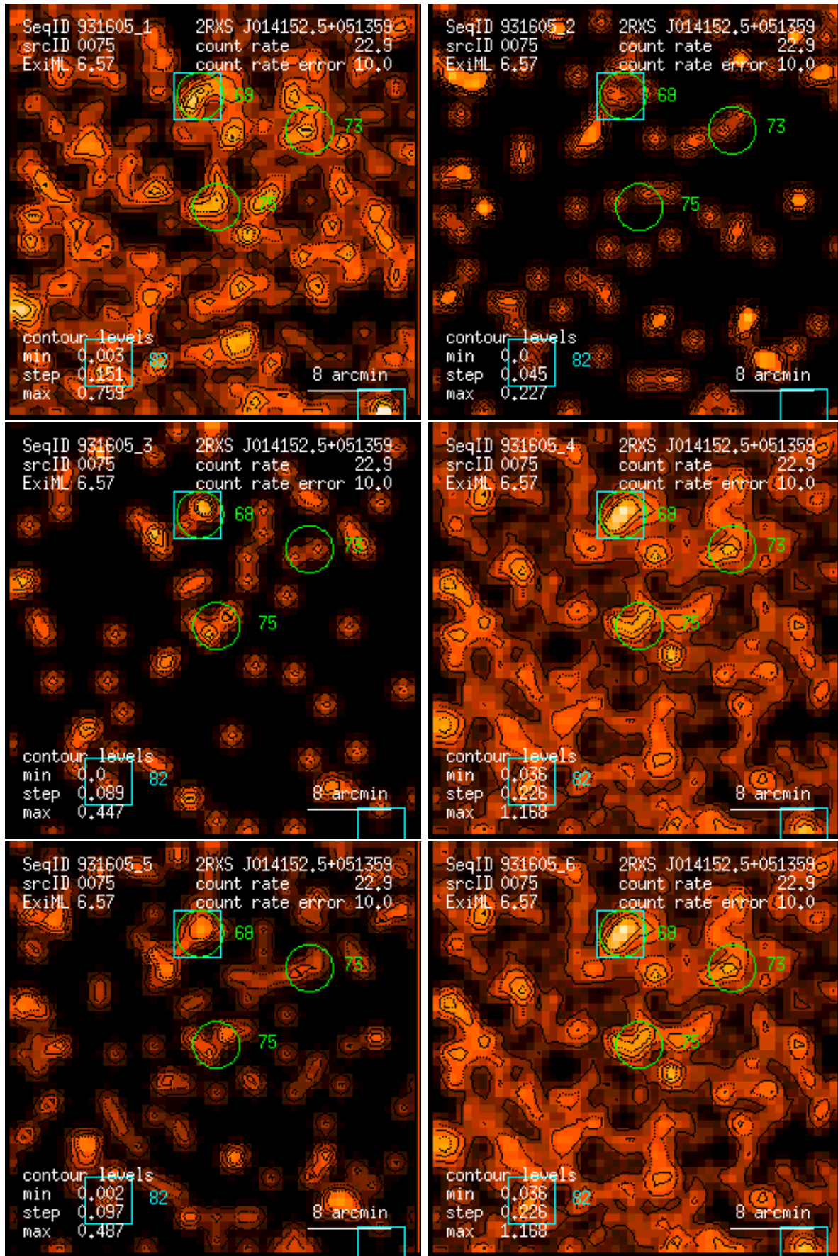
Figure 75: RASS 931605: detection 0075: band rate images, Gaussian filter: (1) PSPC channels 11 – 41, (2) 52 – 90, (3) 91 – 201, (4) 11 – 235, (5) 52 – 201, (6) 11 – 201. Broad band rates in counts/ks. Band rate contour levels in counts/ks/arcmin 2 .
