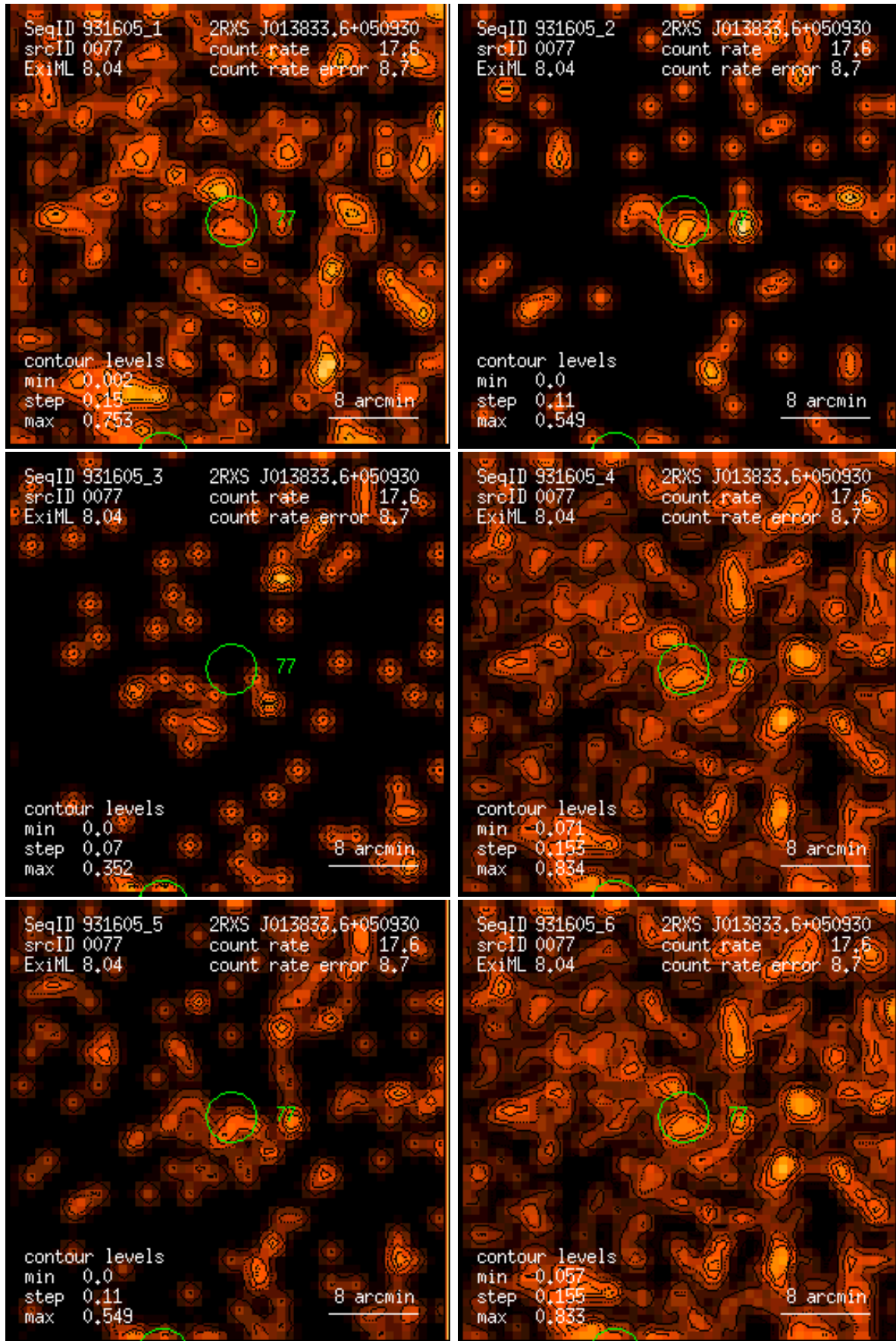
Figure 77: RASS 931605: detection 0077: band rate images, Gaussian filter: (1) PSPC channels 11 – 41, (2) 52 – 90, (3) 91 – 201, (4) 11 – 235, (5) 52 – 201, (6) 11 – 201. Broad band rates in counts/ks. Band rate contour levels in counts/ks/arcmin 2 .
