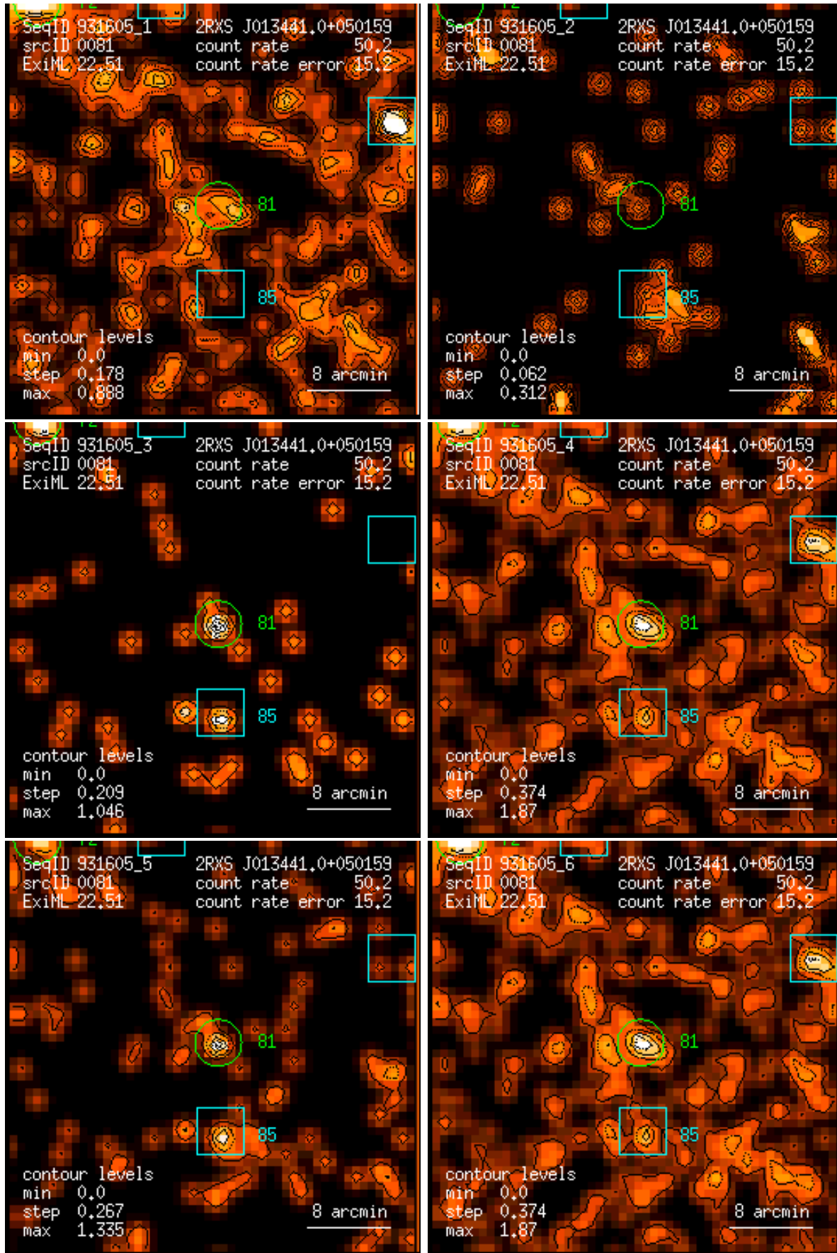
Figure 81: RASS 931605: detection 0081: band rate images, Gaussian filter: (1) PSPC channels 11 – 41, (2) 52 – 90, (3) 91 – 201, (4) 11 – 235, (5) 52 – 201, (6) 11 – 201. Broad band rates in counts/ks. Band rate contour levels in counts/ks/arcmin 2 .
