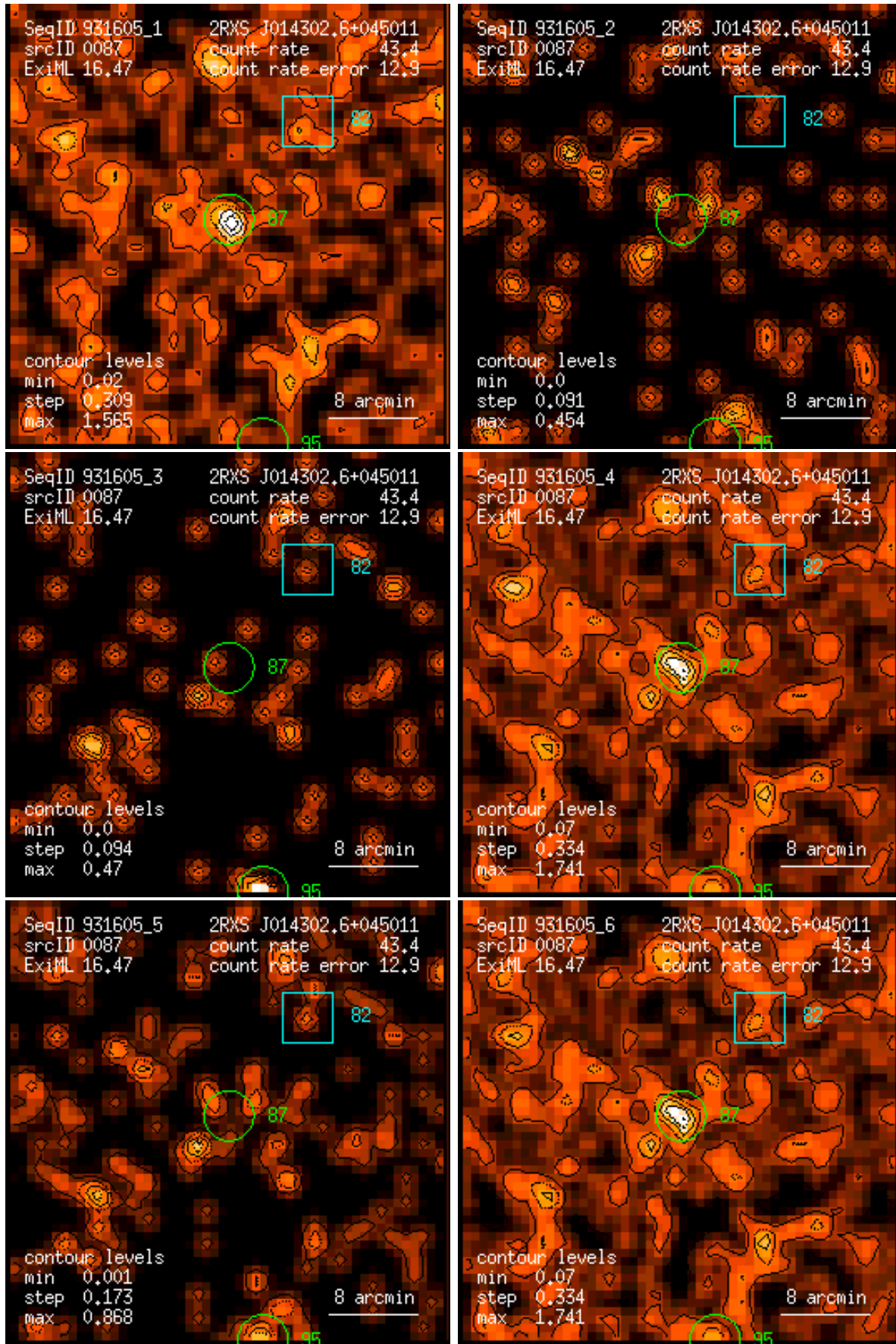
Figure 87: RASS 931605: detection 0087: band rate images, Gaussian filter: (1) PSPC channels 11 – 41, (2) 52 – 90, (3) 91 – 201, (4) 11 – 235, (5) 52 – 201, (6) 11 – 201. Broad band rates in counts/ks. Band rate contour levels in counts/ks/arcmin 2 .
