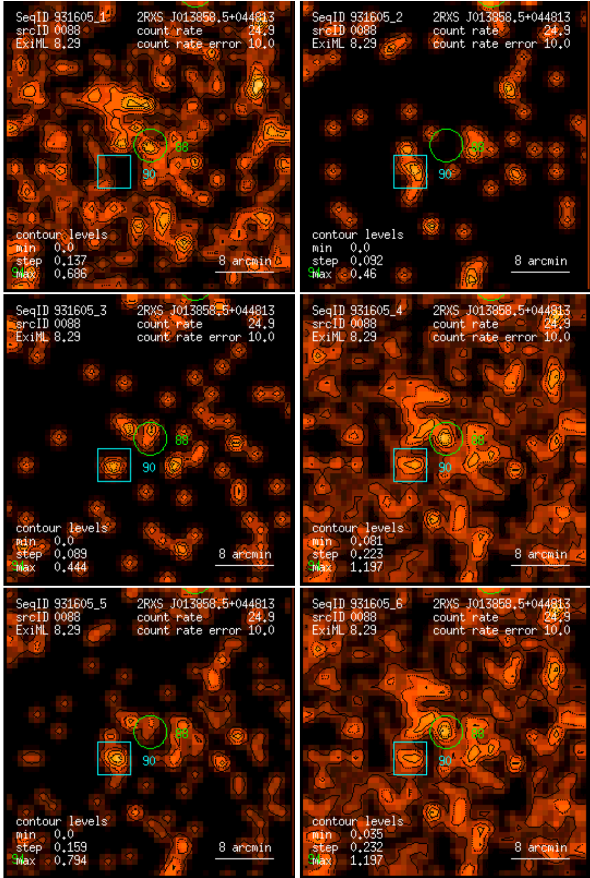
Figure 88: RASS 931605: detection 0088: band rate images, Gaussian filter: (1) PSPC channels 11 – 41, (2) 52 – 90, (3) 91 – 201, (4) 11 – 235, (5) 52 – 201, (6) 11 – 201. Broad band rates in counts/ks. Band rate contour levels in counts/ks/arcmin 2 .
