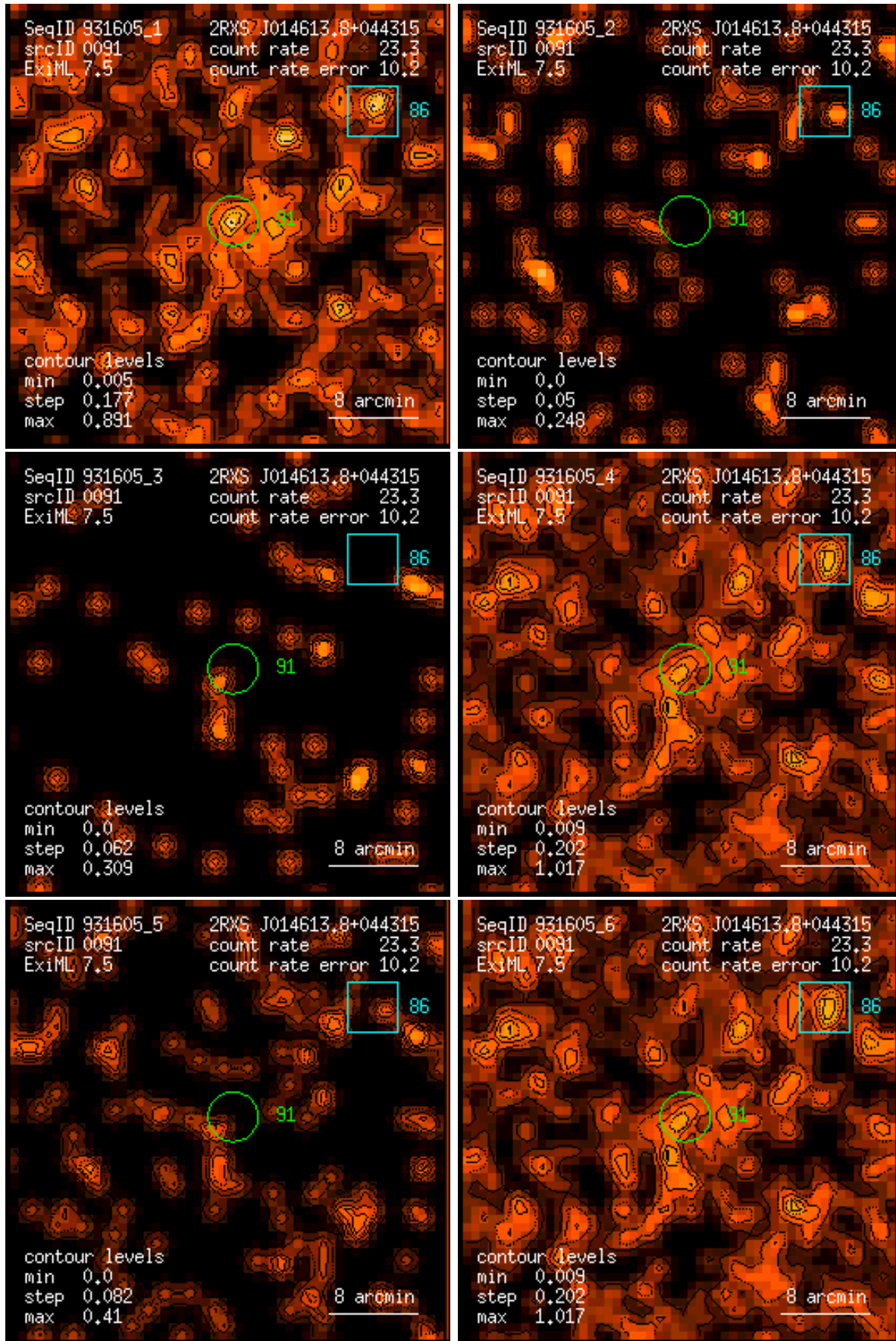
Figure 91: RASS 931605: detection 0091: band rate images, Gaussian filter: (1) PSPC channels 11 – 41, (2) 52 – 90, (3) 91 – 201, (4) 11 – 235, (5) 52 – 201, (6) 11 – 201. Broad band rates in counts/ks. Band rate contour levels in counts/ks/arcmin 2 .
