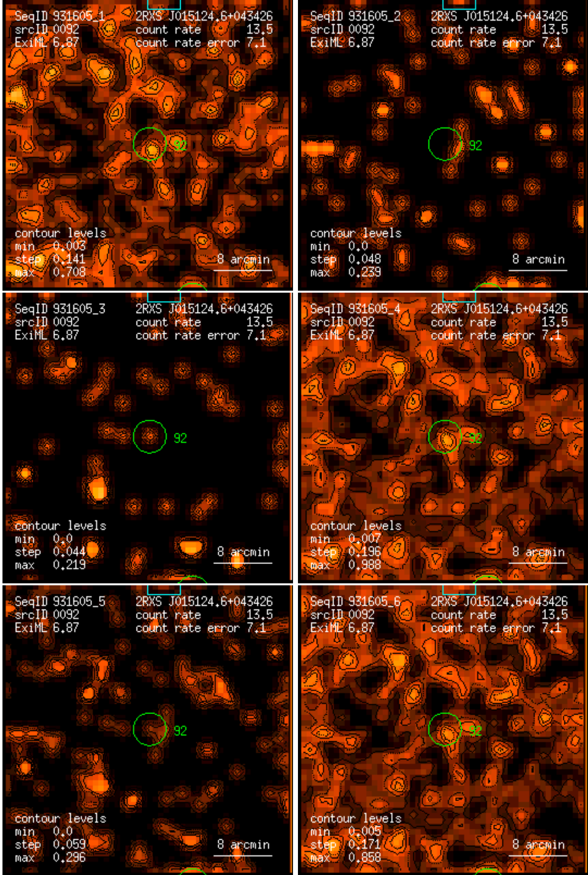
Figure 92: RASS 931605: detection 0092: band rate images, Gaussian filter: (1) PSPC channels 11 – 41, (2) 52 – 90, (3) 91 – 201, (4) 11 – 235, (5) 52 – 201, (6) 11 – 201. Broad band rates in counts/ks. Band rate contour levels in counts/ks/arcmin 2 .
