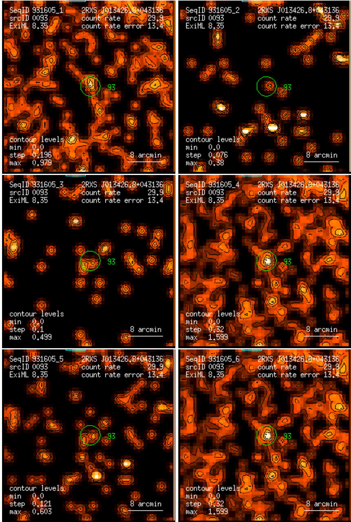
Figure 93: RASS 931605: detection 0093: band rate images, Gaussian filter: (1) PSPC channels 11 – 41, (2) 52 – 90, (3) 91 – 201, (4) 11 – 235, (5) 52 – 201, (6) 11 – 201. Broad band rates in counts/ks. Band rate contour levels in counts/ks/arcmin 2 .
