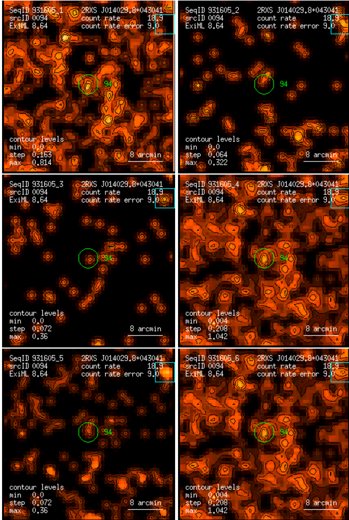
Figure 94: RASS 931605: detection 0094: band rate images, Gaussian filter: (1) PSPC channels 11 – 41, (2) 52 – 90, (3) 91 – 201, (4) 11 – 235, (5) 52 – 201, (6) 11 – 201. Broad band rates in counts/ks. Band rate contour levels in counts/ks/arcmin 2 .
