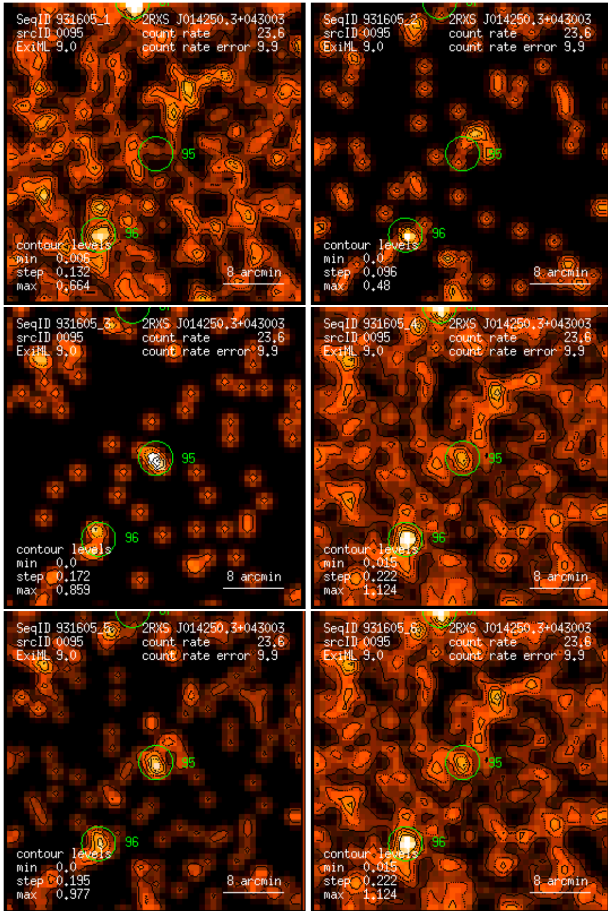
Figure 95: RASS 931605: detection 0095: band rate images, Gaussian filter: (1) PSPC channels 11 – 41, (2) 52 – 90, (3) 91 – 201, (4) 11 – 235, (5) 52 – 201, (6) 11 – 201. Broad band rates in counts/ks. Band rate contour levels in counts/ks/arcmin 2 .
