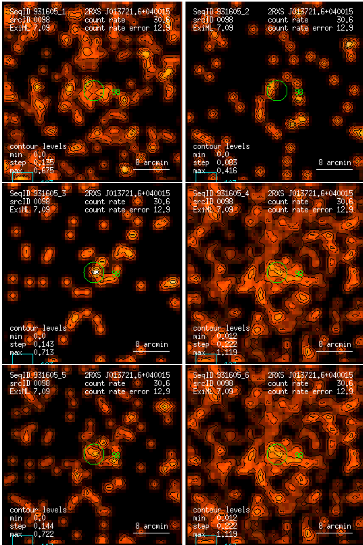
Figure 98: RASS 931605: detection 0098: band rate images, Gaussian filter: (1) PSPC channels 11 – 41, (2) 52 – 90, (3) 91 – 201, (4) 11 – 235, (5) 52 – 201, (6) 11 – 201. Broad band rates in counts/ks. Band rate contour levels in counts/ks/arcmin 2 .
