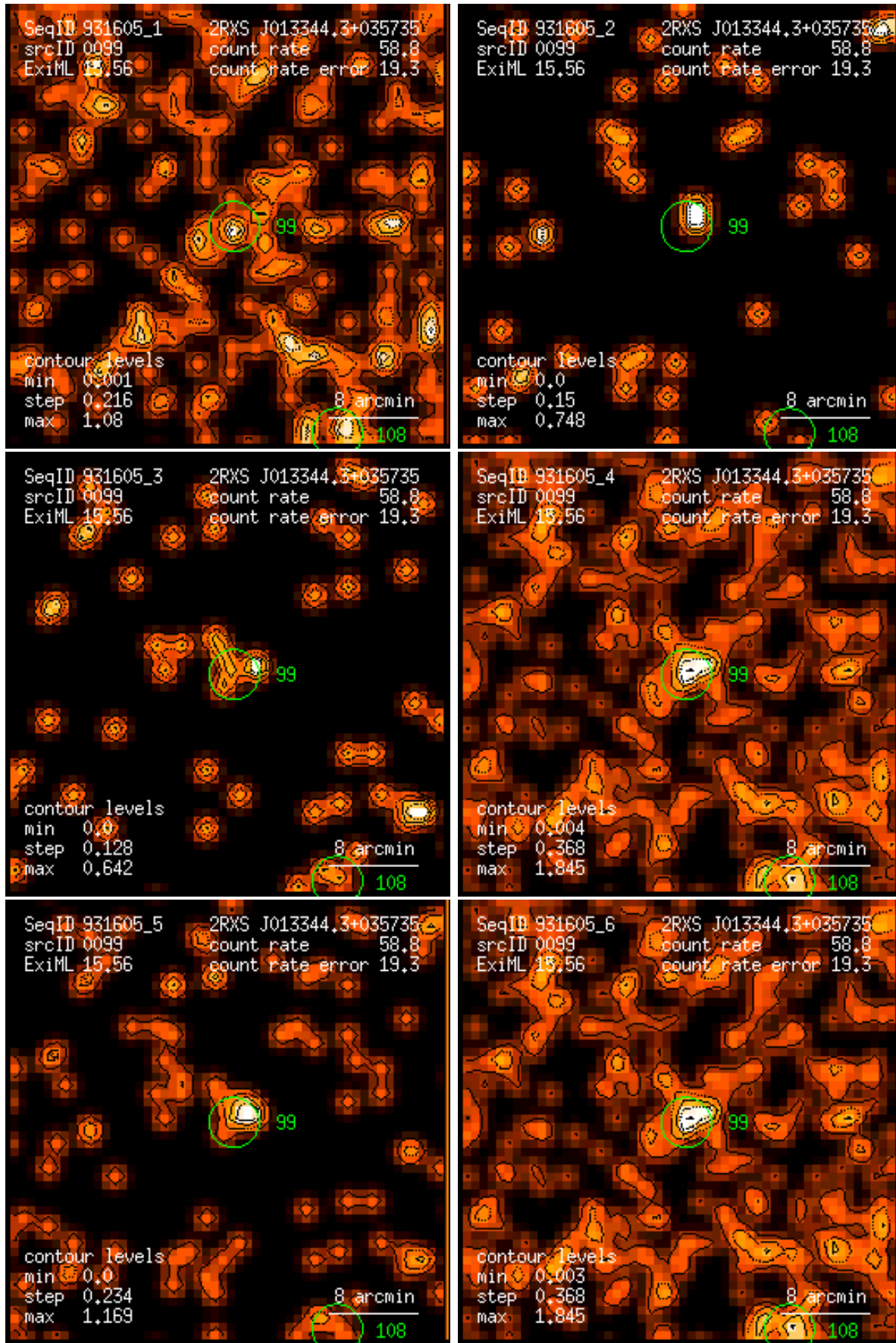
Figure 99: RASS 931605: detection 0099: band rate images, Gaussian filter: (1) PSPC channels 11 – 41, (2) 52 – 90, (3) 91 – 201, (4) 11 – 235, (5) 52 – 201, (6) 11 – 201. Broad band rates in counts/ks. Band rate contour levels in counts/ks/arcmin 2 .
