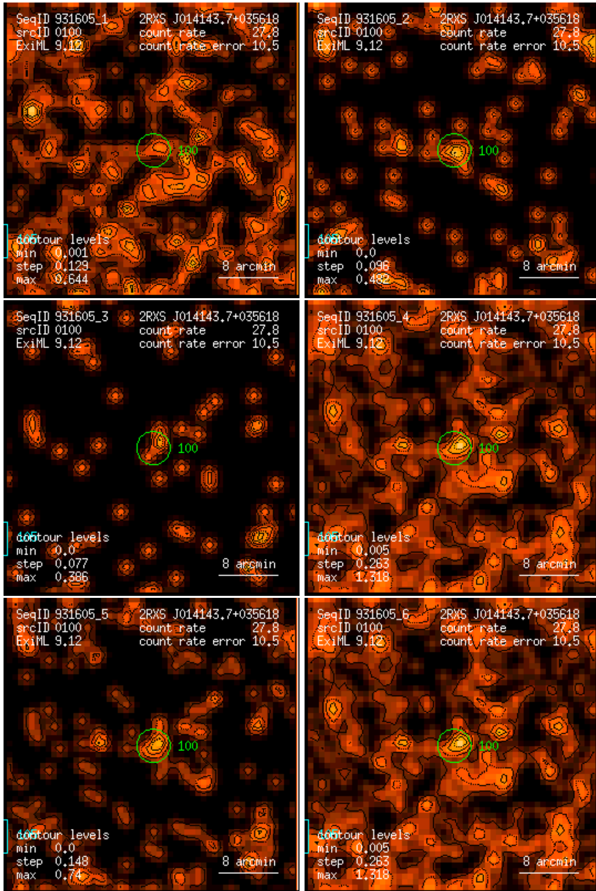
Figure 100: RASS 931605: detection 0100: band rate images, Gaussian filter: (1) PSPC channels 11 – 41, (2) 52 – 90, (3) 91 – 201, (4) 11 – 235, (5) 52 – 201, (6) 11 – 201. Broad band rates in counts/ks. Band rate contour levels in counts/ks/arcmin 2 .
