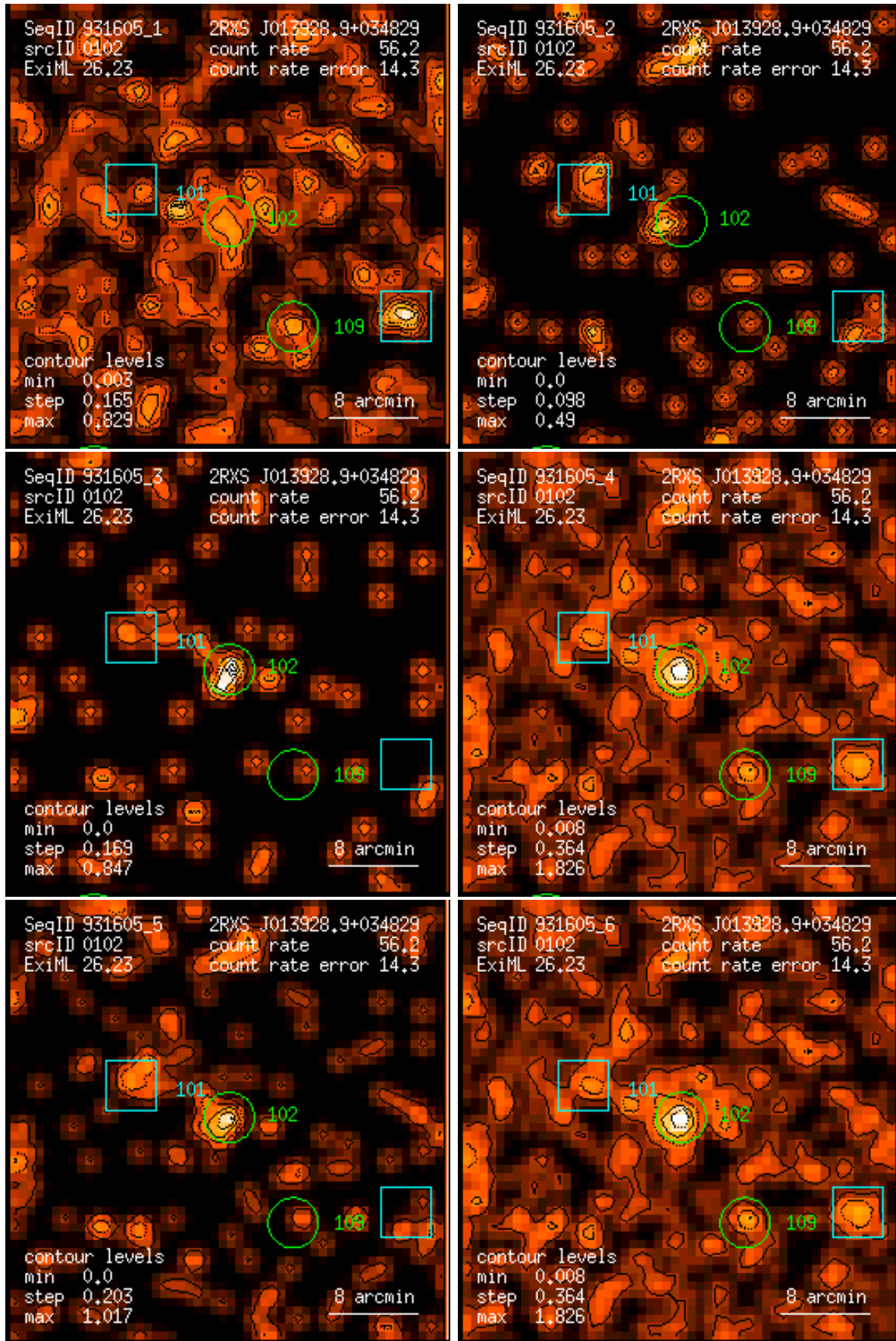
Figure 102: RASS 931605: detection 0102: band rate images, Gaussian filter: (1) PSPC channels 11 – 41, (2) 52 – 90, (3) 91 – 201, (4) 11 – 235, (5) 52 – 201, (6) 11 – 201. Broad band rates in counts/ks. Band rate contour levels in counts/ks/arcmin 2 .
