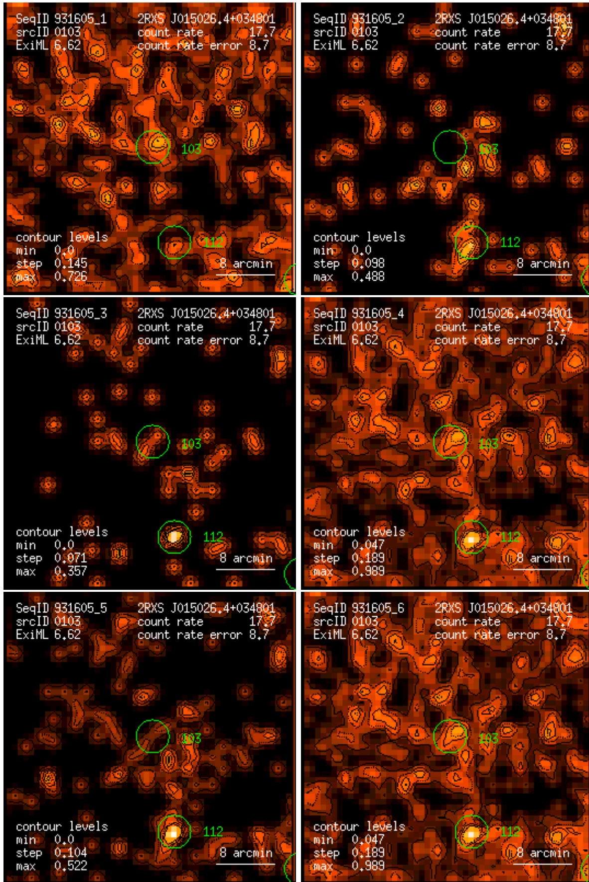
Figure 103: RASS 931605: detection 0103: band rate images, Gaussian filter: (1) PSPC channels 11 – 41, (2) 52 – 90, (3) 91 – 201, (4) 11 – 235, (5) 52 – 201, (6) 11 – 201. Broad band rates in counts/ks. Band rate contour levels in counts/ks/arcmin 2 .
