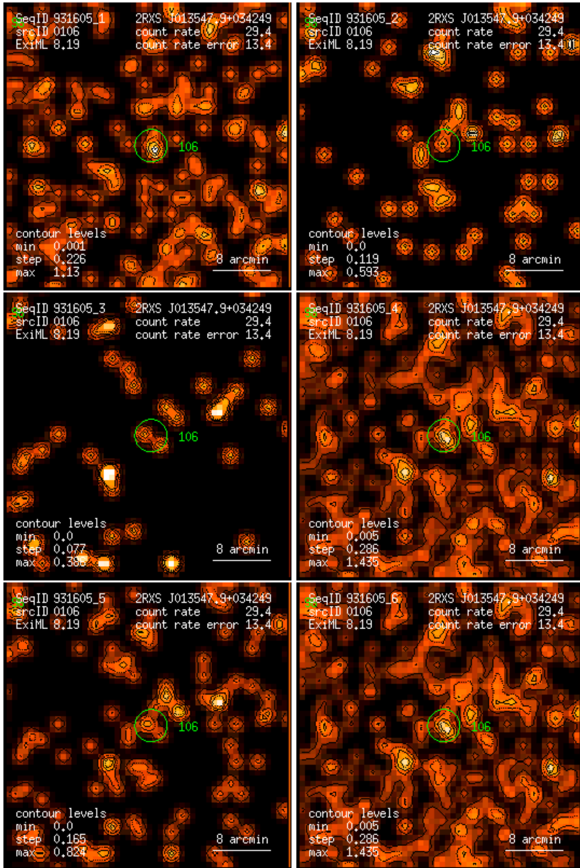
Figure 106: RASS 931605: detection 0106: band rate images, Gaussian filter: (1) PSPC channels 11 – 41, (2) 52 – 90, (3) 91 – 201, (4) 11 – 235, (5) 52 – 201, (6) 11 – 201. Broad band rates in counts/ks. Band rate contour levels in counts/ks/arcmin 2 .
