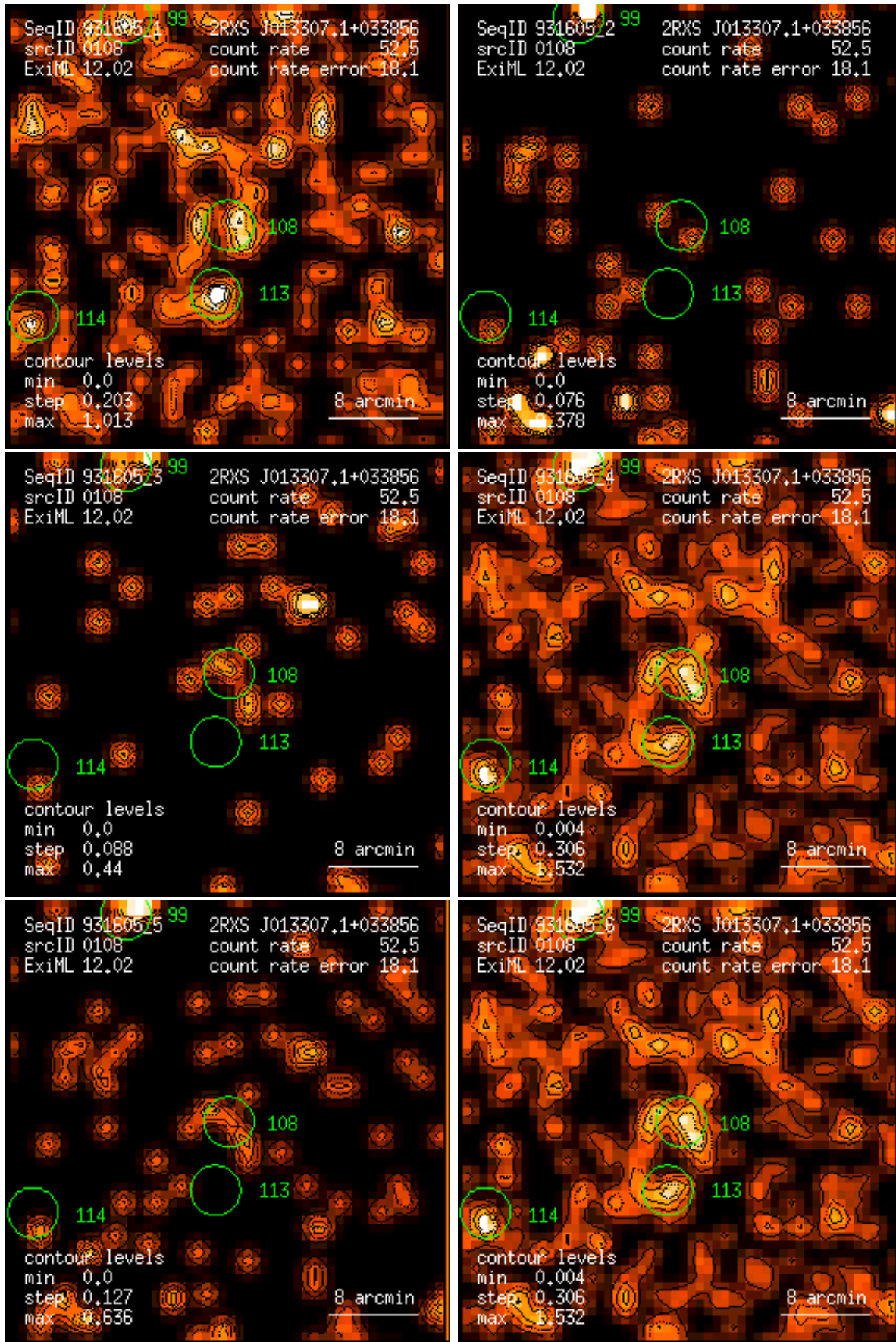
Figure 108: RASS 931605: detection 0108: band rate images, Gaussian filter: (1) PSPC channels 11 – 41, (2) 52 – 90, (3) 91 – 201, (4) 11 – 235, (5) 52 – 201, (6) 11 – 201. Broad band rates in counts/ks. Band rate contour levels in counts/ks/arcmin 2 .
