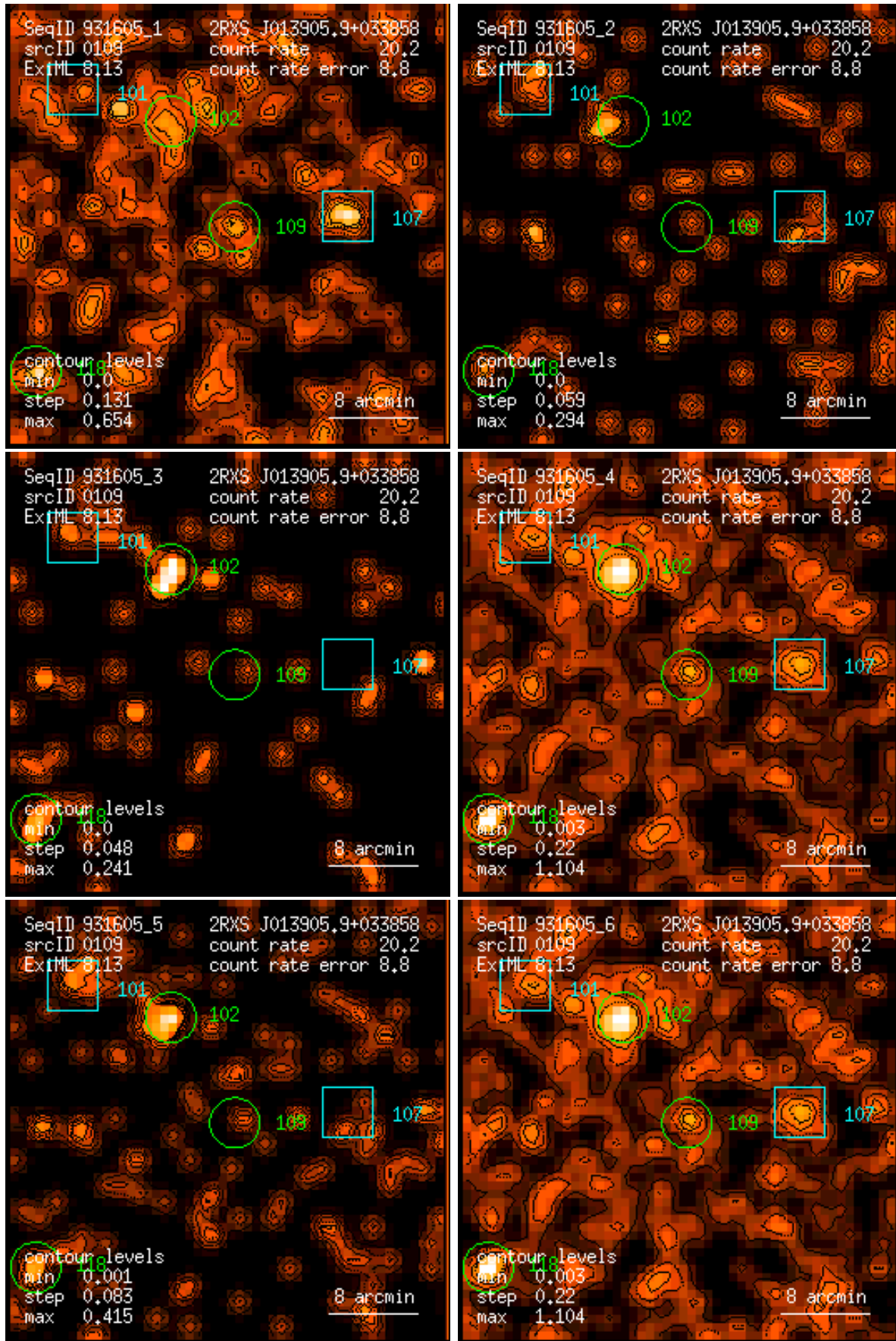
Figure 109: RASS 931605: detection 0109: band rate images, Gaussian filter: (1) PSPC channels 11 – 41, (2) 52 – 90, (3) 91 – 201, (4) 11 – 235, (5) 52 – 201, (6) 11 – 201. Broad band rates in counts/ks. Band rate contour levels in counts/ks/arcmin 2 .
