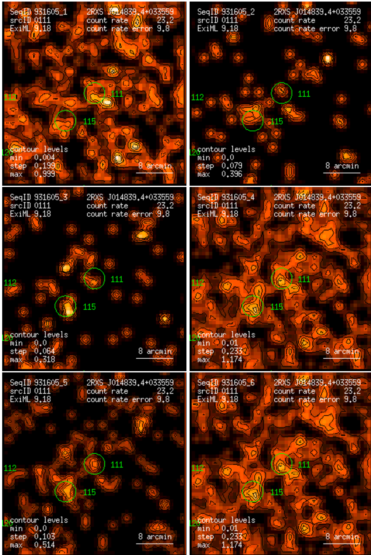
Figure 111: RASS 931605: detection 0111: band rate images, Gaussian filter: (1) PSPC channels 11 – 41, (2) 52 – 90, (3) 91 – 201, (4) 11 – 235, (5) 52 – 201, (6) 11 – 201. Broad band rates in counts/ks. Band rate contour levels in counts/ks/arcmin 2 .
