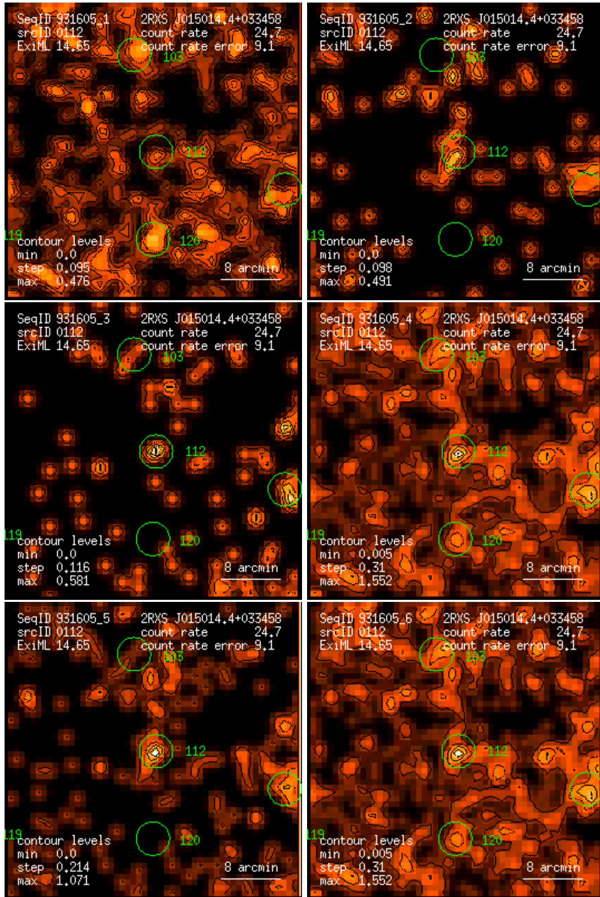
Figure 112: RASS 931605: detection 0112: band rate images, Gaussian filter: (1) PSPC channels 11 – 41, (2) 52 – 90, (3) 91 – 201, (4) 11 – 235, (5) 52 – 201, (6) 11 – 201. Broad band rates in counts/ks. Band rate contour levels in counts/ks/arcmin 2 .
