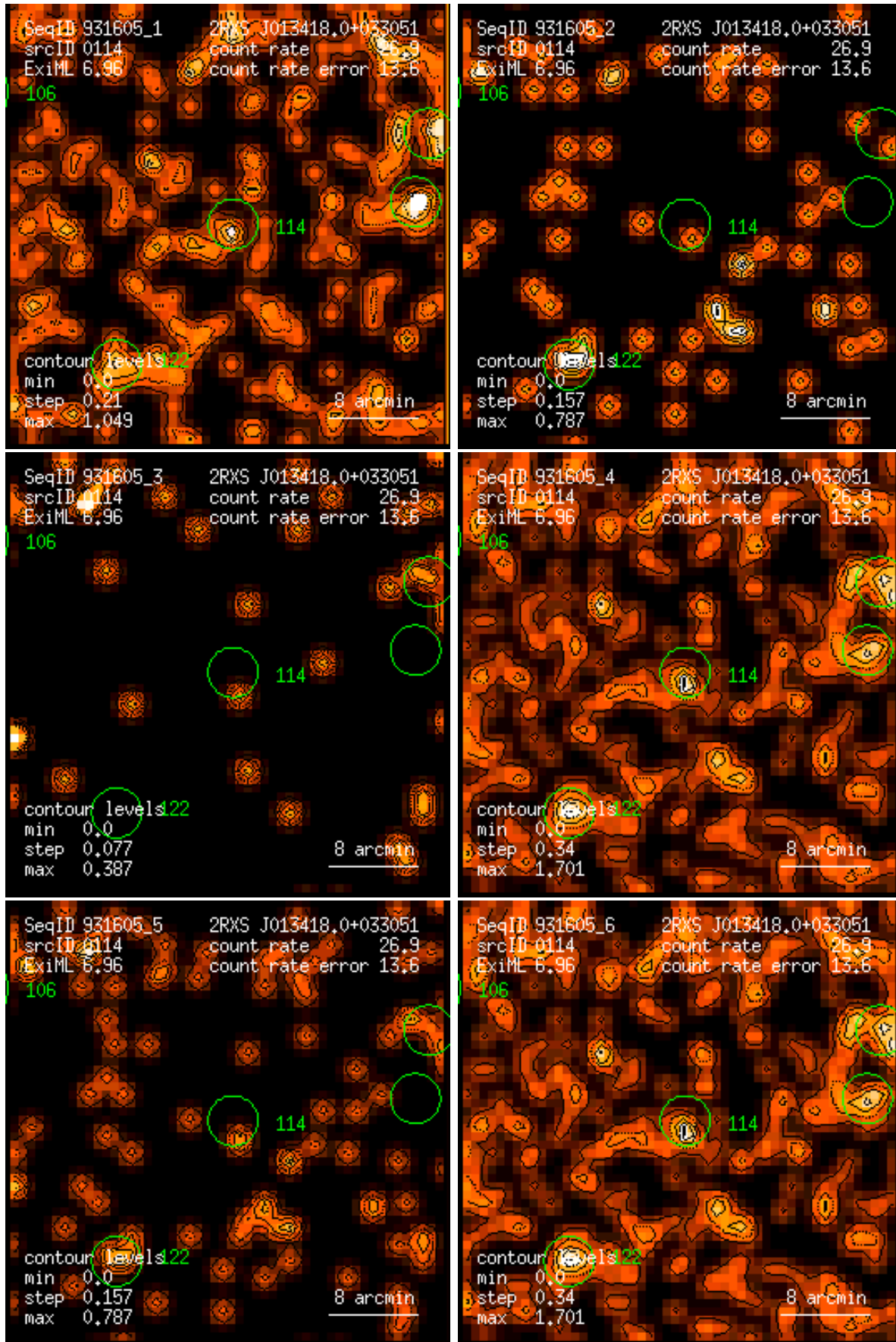
Figure 114: RASS 931605: detection 0114: band rate images, Gaussian filter: (1) PSPC channels 11 – 41, (2) 52 – 90, (3) 91 – 201, (4) 11 – 235, (5) 52 – 201, (6) 11 – 201. Broad band rates in counts/ks. Band rate contour levels in counts/ks/arcmin 2 .
