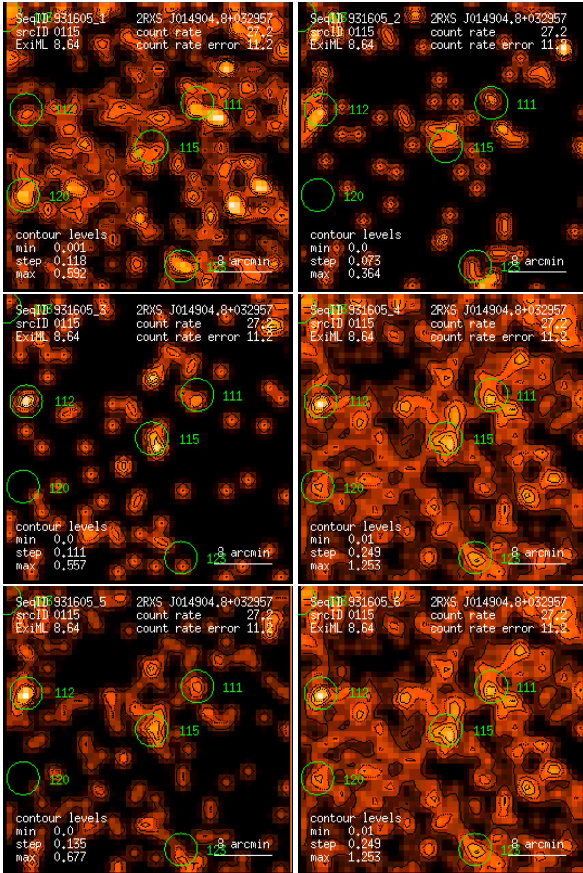
Figure 115: RASS 931605: detection 0115: band rate images, Gaussian filter: (1) PSPC channels 11 – 41, (2) 52 – 90, (3) 91 – 201, (4) 11 – 235, (5) 52 – 201, (6) 11 – 201. Broad band rates in counts/ks. Band rate contour levels in counts/ks/arcmin 2 .
