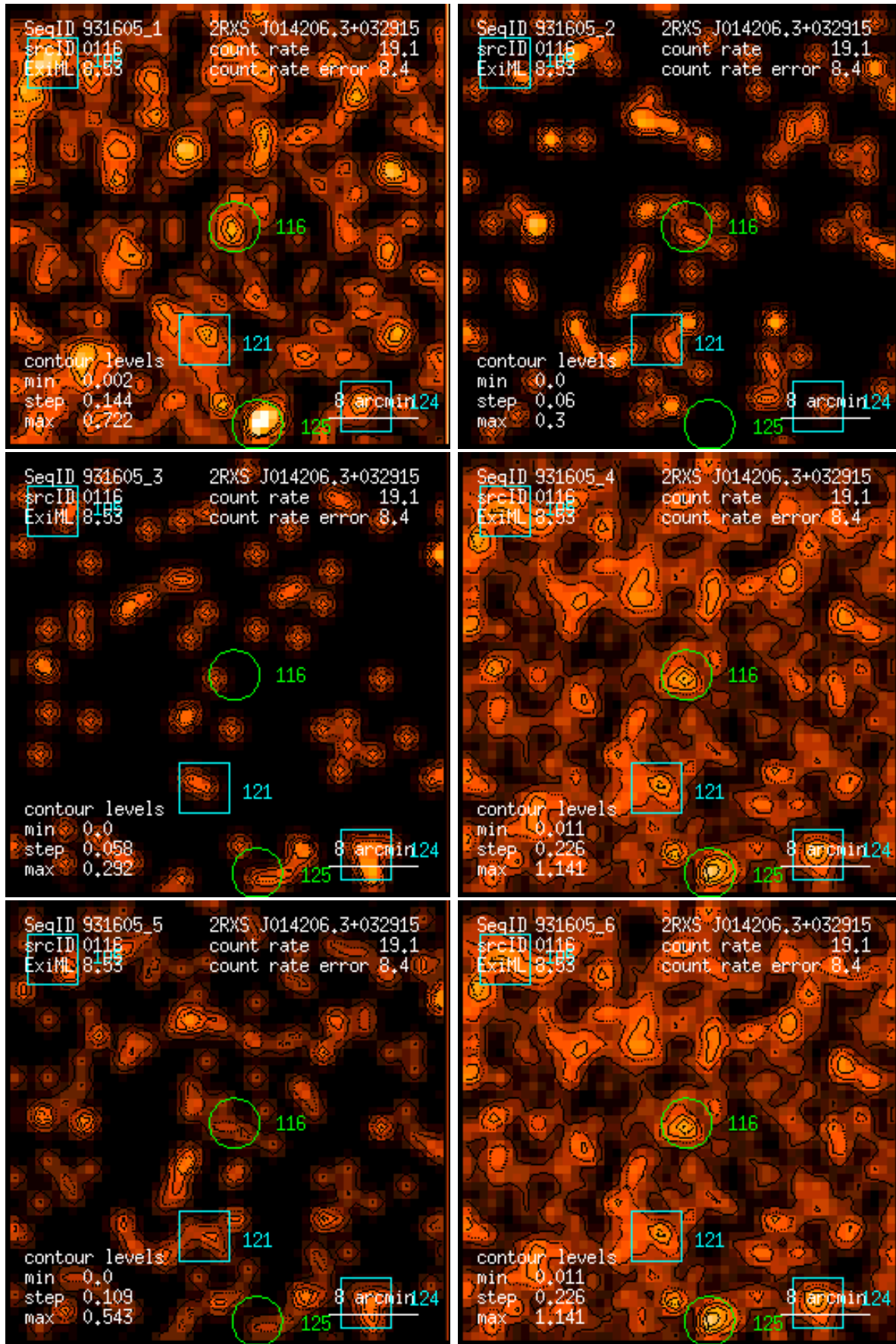
Figure 116: RASS 931605: detection 0116: band rate images, Gaussian filter: (1) PSPC channels 11 – 41, (2) 52 – 90, (3) 91 – 201, (4) 11 – 235, (5) 52 – 201, (6) 11 – 201. Broad band rates in counts/ks. Band rate contour levels in counts/ks/arcmin 2 .
