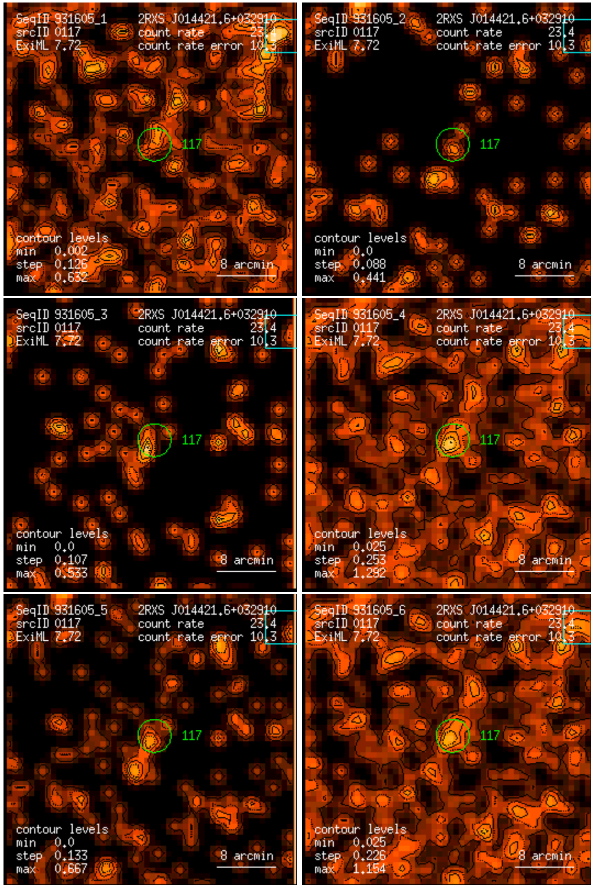
Figure 117: RASS 931605: detection 0117: band rate images, Gaussian filter: (1) PSPC channels 11 – 41, (2) 52 – 90, (3) 91 – 201, (4) 11 – 235, (5) 52 – 201, (6) 11 – 201. Broad band rates in counts/ks. Band rate contour levels in counts/ks/arcmin 2 .
