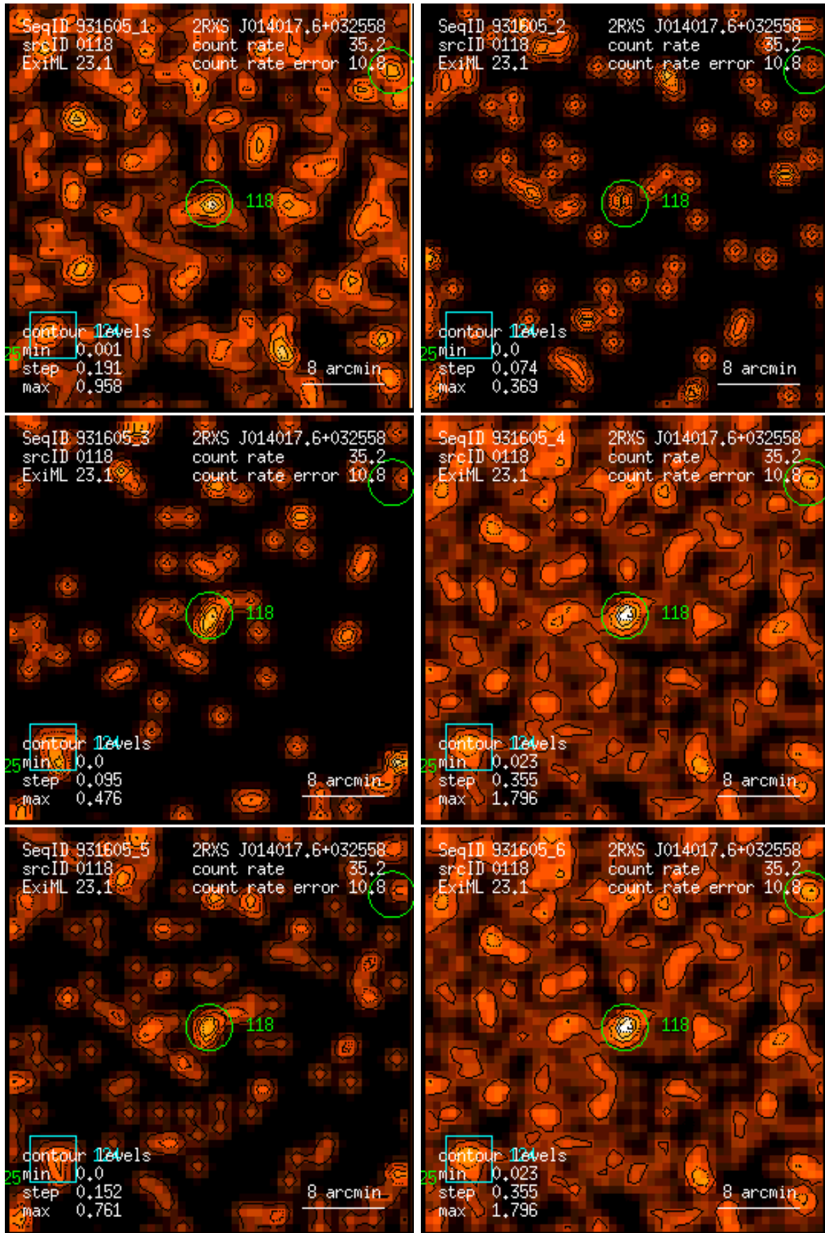
Figure 118: RASS 931605: detection 0118: band rate images, Gaussian filter: (1) PSPC channels 11 – 41, (2) 52 – 90, (3) 91 – 201, (4) 11 – 235, (5) 52 – 201, (6) 11 – 201. Broad band rates in counts/ks. Band rate contour levels in counts/ks/arcmin 2 .
