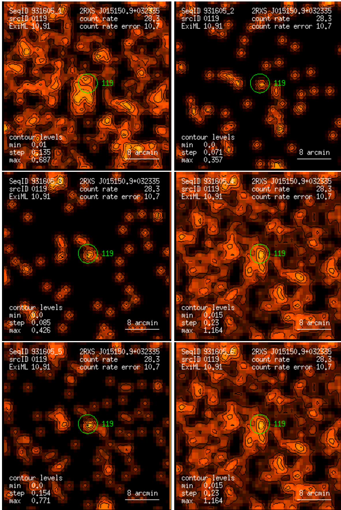
Figure 119: RASS 931605: detection 0119: band rate images, Gaussian filter: (1) PSPC channels 11 – 41, (2) 52 – 90, (3) 91 – 201, (4) 11 – 235, (5) 52 – 201, (6) 11 – 201. Broad band rates in counts/ks. Band rate contour levels in counts/ks/arcmin 2 .
