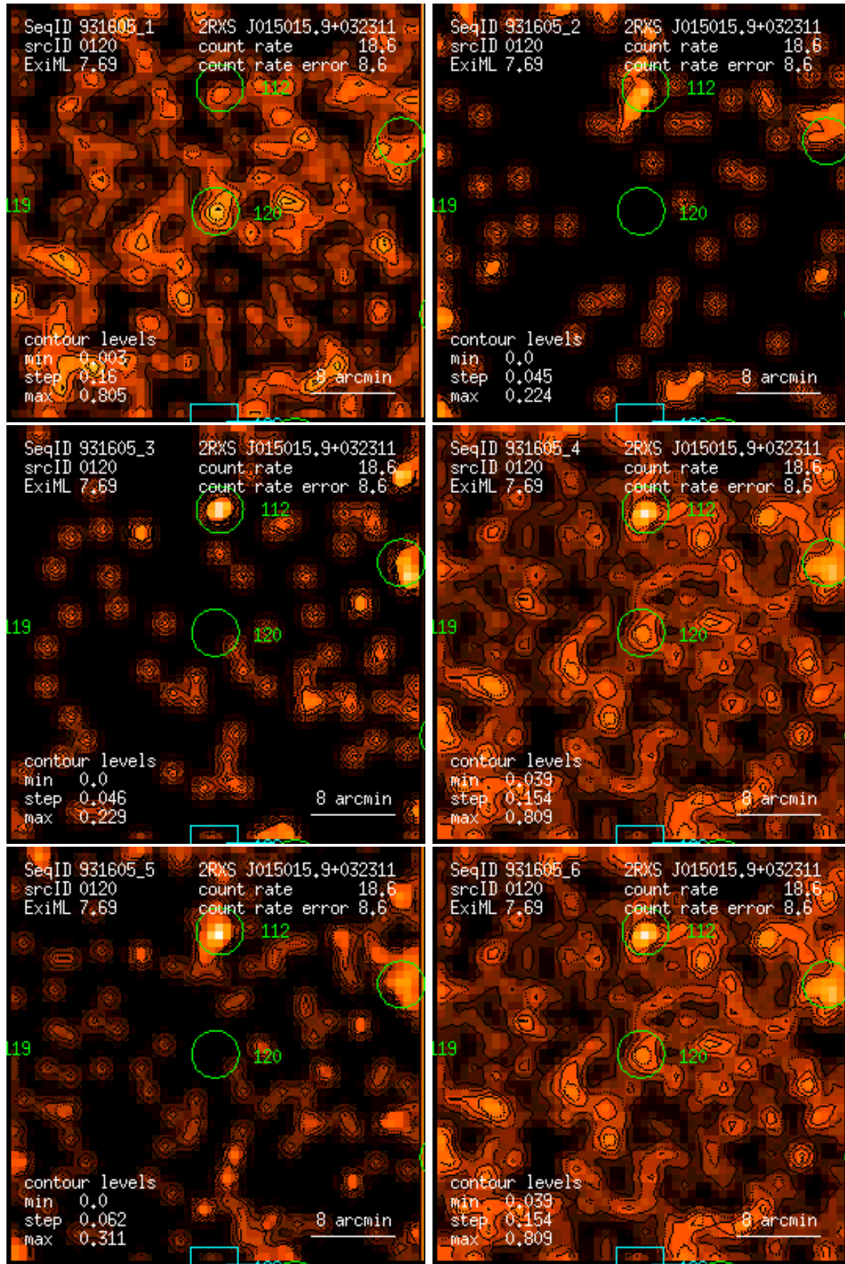
Figure 120: RASS 931605: detection 0120: band rate images, Gaussian filter: (1) PSPPC channels 11 – 41, (2) 52 – 90, (3) 91 – 201, (4) 11 – 235, (5) 52 – 201, (6) 11 – 201. Broad band rates in counts/ks. Band rate contour levels in counts/ks/arcmin 2 .
