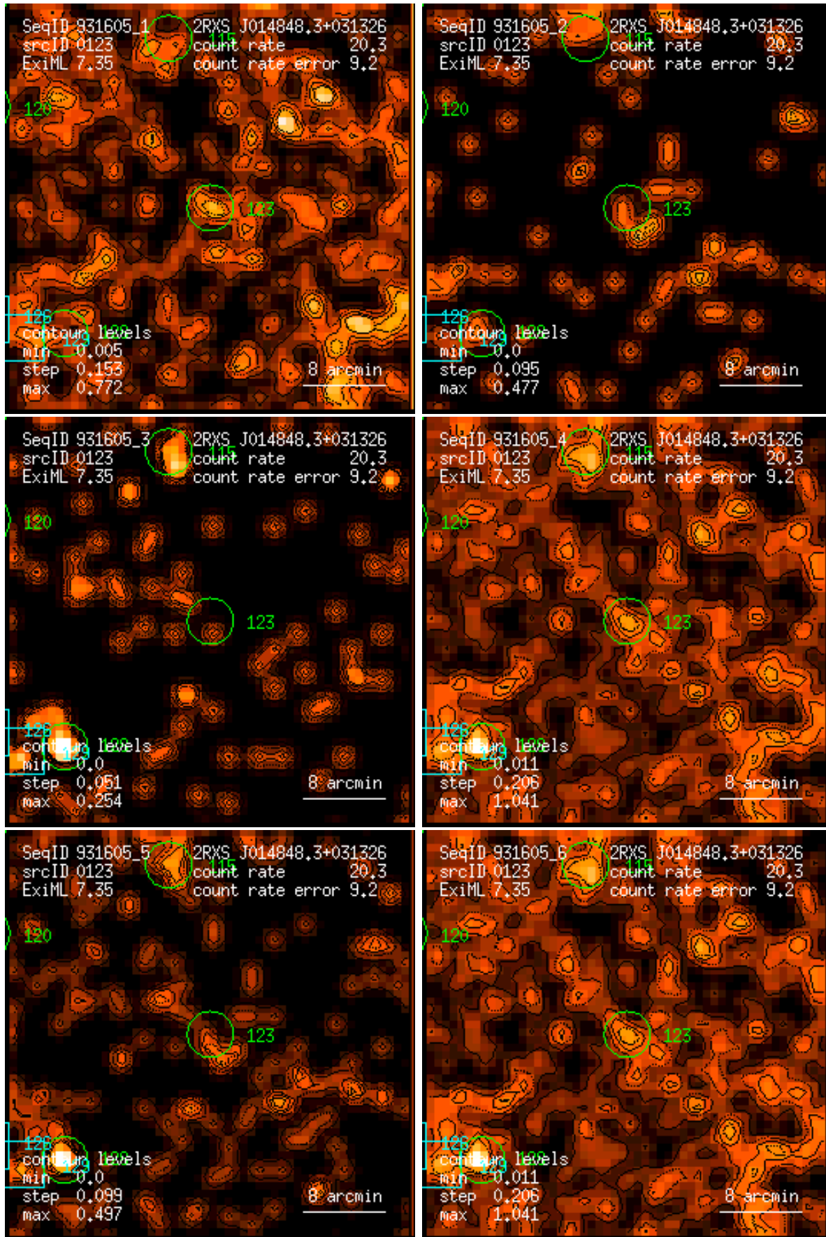
Figure 123: RASS 931605: detection 0123: band rate images, Gaussian filter: (1) PSPC channels 11 – 41, (2) 52 – 90, (3) 91 – 201, (4) 11 – 235, (5) 52 – 201, (6) 11 – 201. Broad band rates in counts/ks. Band rate contour levels in counts/ks/arcmin 2 .
