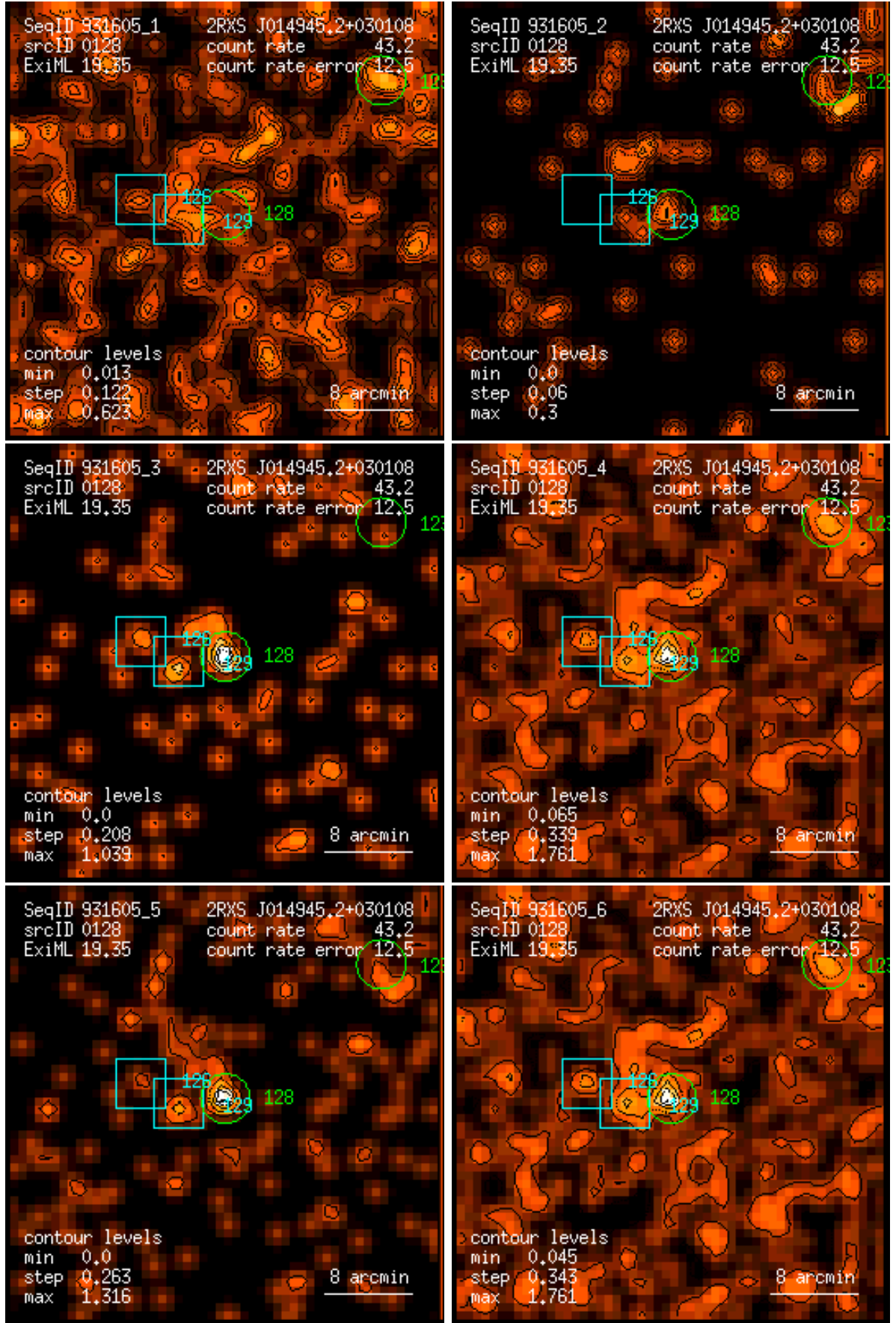
Figure 128: RASS 931605: detection 0128: band rate images, Gaussian filter: (1) PSPC channels 11 – 41, (2) 52 – 90, (3) 91 – 201, (4) 11 – 235, (5) 52 – 201, (6) 11 – 201. Broad band rates in counts/ks. Band rate contour levels in counts/ks/arcmin 2 .
