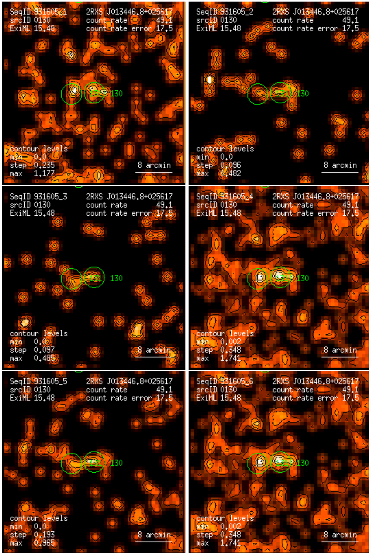
Figure 130: RASS 931605: detection 0130: band rate images, Gaussian filter: (1) PSPC channels 11 – 41, (2) 52 – 90, (3) 91 – 201, (4) 11 – 235, (5) 52 – 201, (6) 11 – 201. Broad band rates in counts/ks. Band rate contour levels in counts/ks/arcmin 2 .
