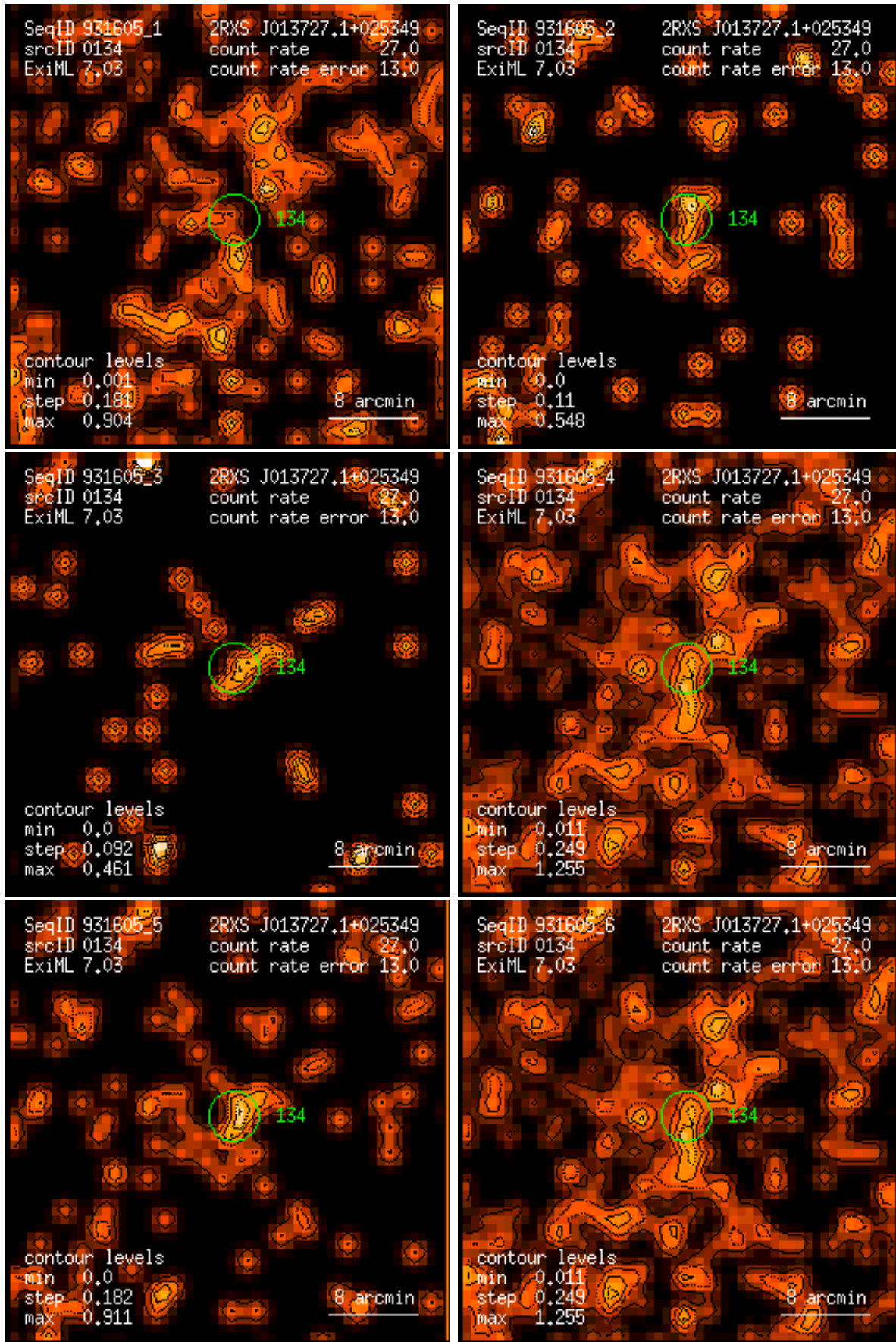
Figure 134: RASS 931605: detection 0134: band rate images, Gaussian filter: (1) PSPC channels 11 – 41, (2) 52 – 90, (3) 91 – 201, (4) 11 – 235, (5) 52 – 201, (6) 11 – 201. Broad band rates in counts/ks. Band rate contour levels in counts/ks/arcmin 2 .
