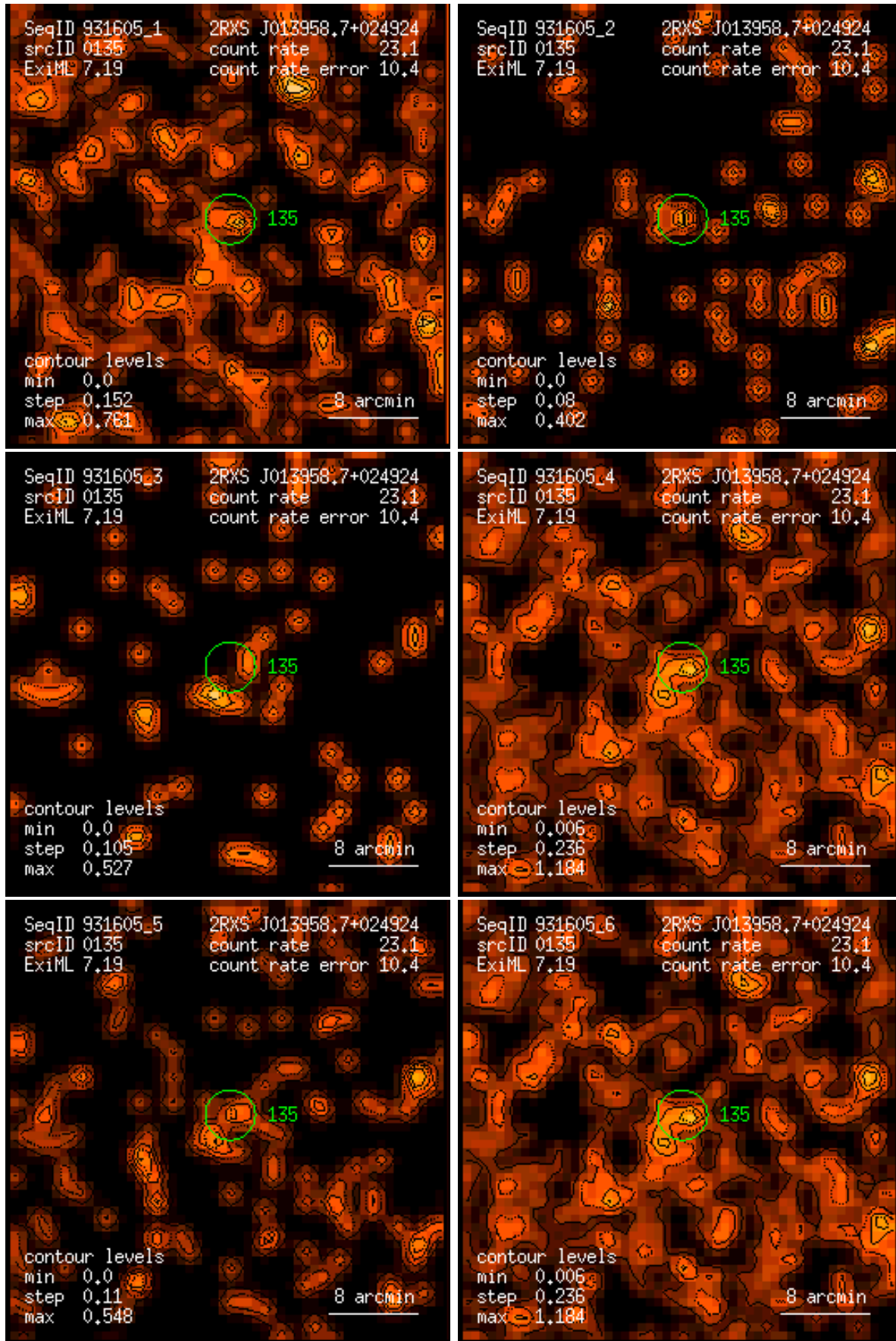
Figure 135: RASS 931605: detection 0135: band rate images, Gaussian filter: (1) PSPC channels 11 – 41, (2) 52 – 90, (3) 91 – 201, (4) 11 – 235, (5) 52 – 201, (6) 11 – 201. Broad band rates in counts/ks. Band rate contour levels in counts/ks/arcmin 2 .
