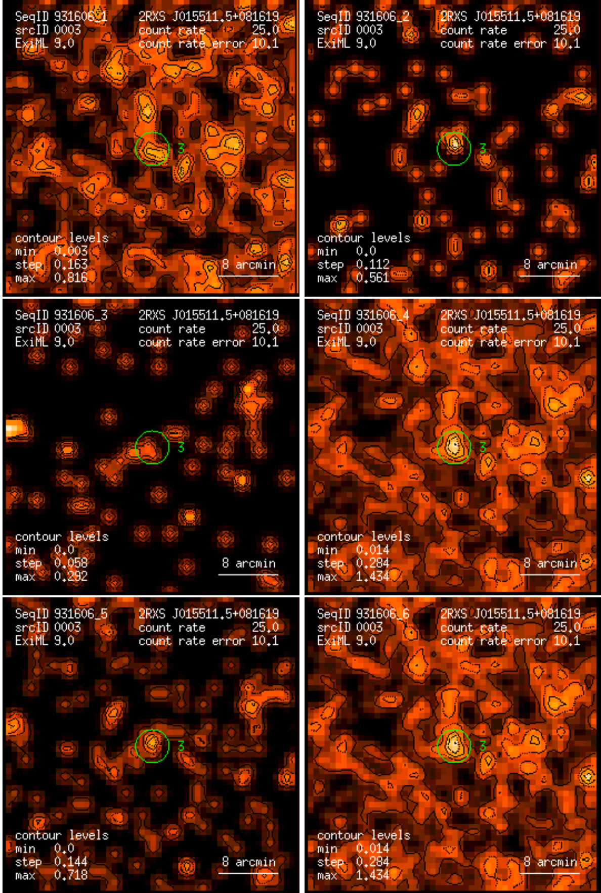
Figure 3: RASS 931606: detection 0003: band rate images, Gaussian filter: (1) PSPC channels 11 – 41, (2) 52 – 90, (3) 91 – 201, (4) 11 – 235, (5) 52 – 201, (6) 11 – 201. Broad band rates in counts/ks. Band rate contour levels in counts/ks/arcmin 2 .
