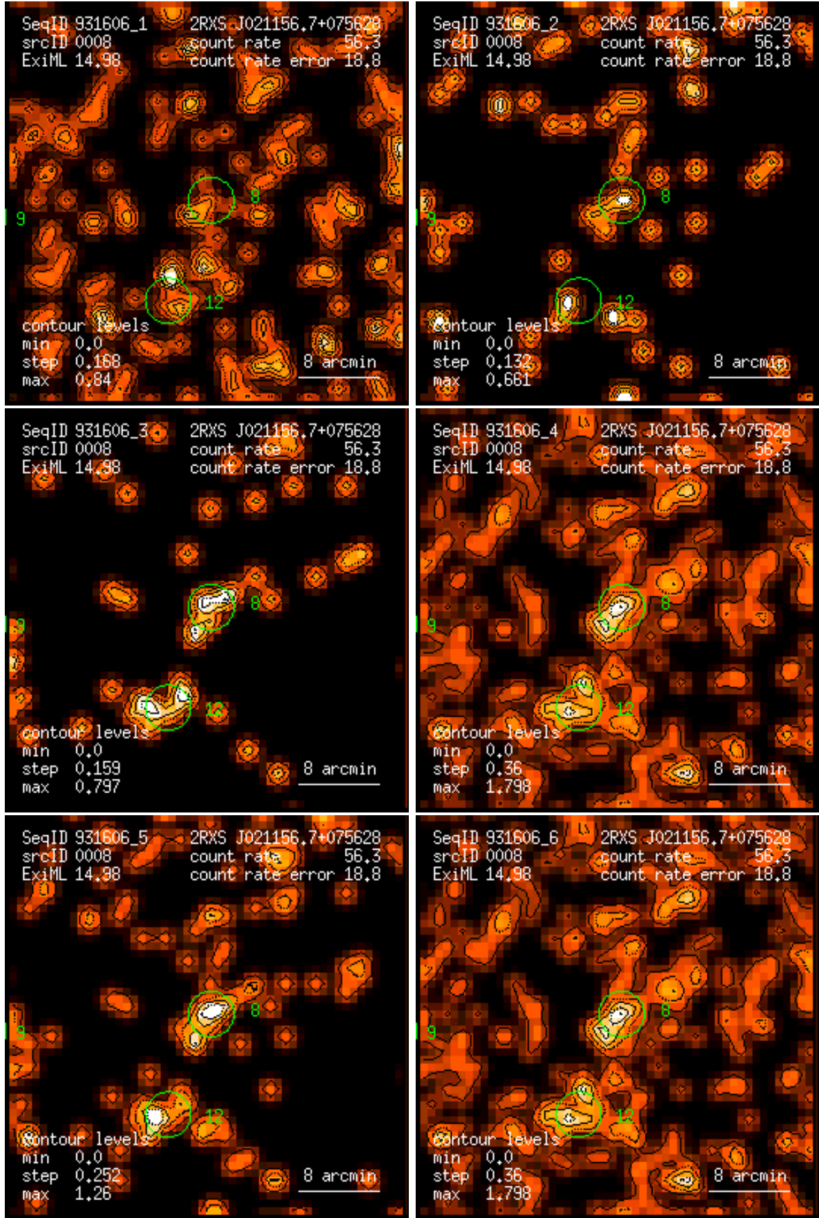
Figure 8: RASS 931606: detection 0008: band rate images, Gaussian filter: (1) PSPC channels 11 – 41, (2) 52 – 90, (3) 91 – 201, (4) 11 – 235, (5) 52 – 201, (6) 11 – 201. Broad band rates in counts/ks. Band rate contour levels in counts/ks/arcmin 2 .
