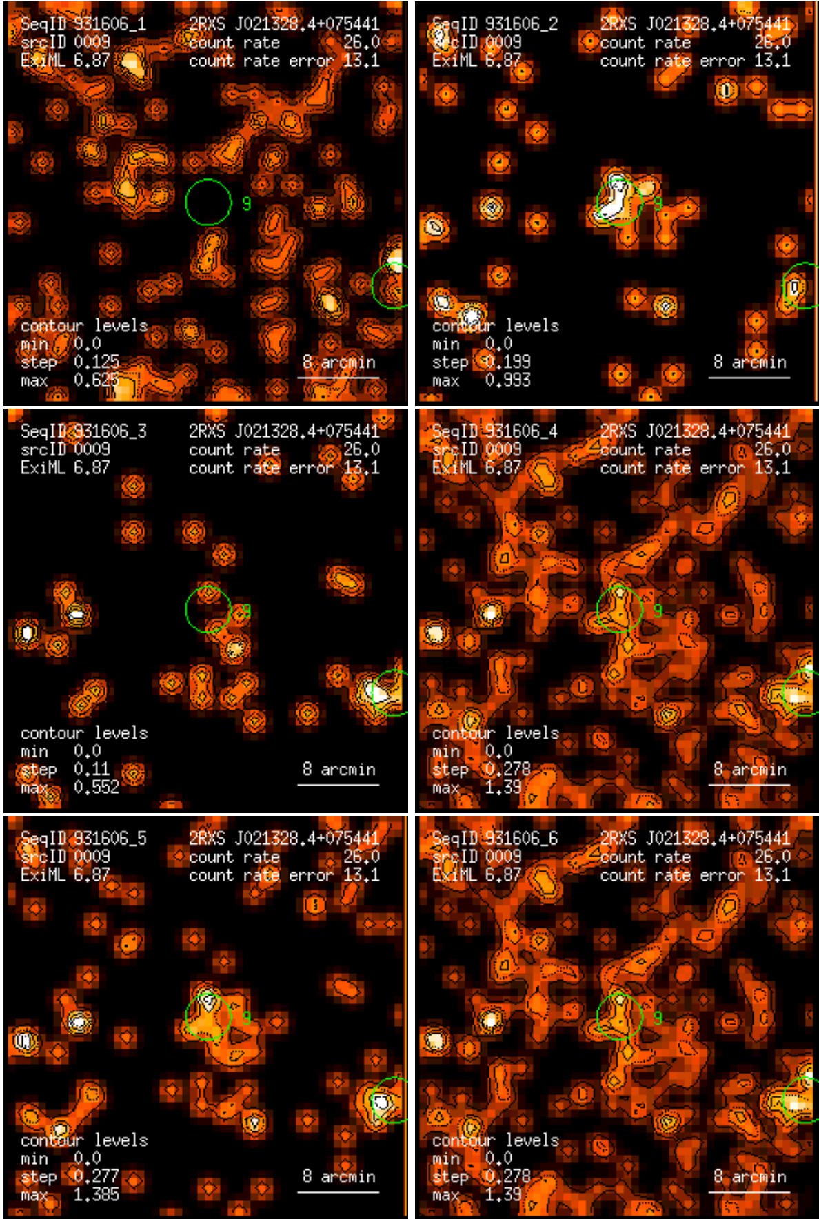
Figure 9: RASS 931606: detection 0009: band rate images, Gaussian filter: (1) PSPC channels 11 – 41, (2) 52 – 90, (3) 91 – 201, (4) 11 – 235, (5) 52 – 201, (6) 11 – 201. Broad band rates in counts/ks. Band rate contour levels in counts/ks/arcmin 2 .
