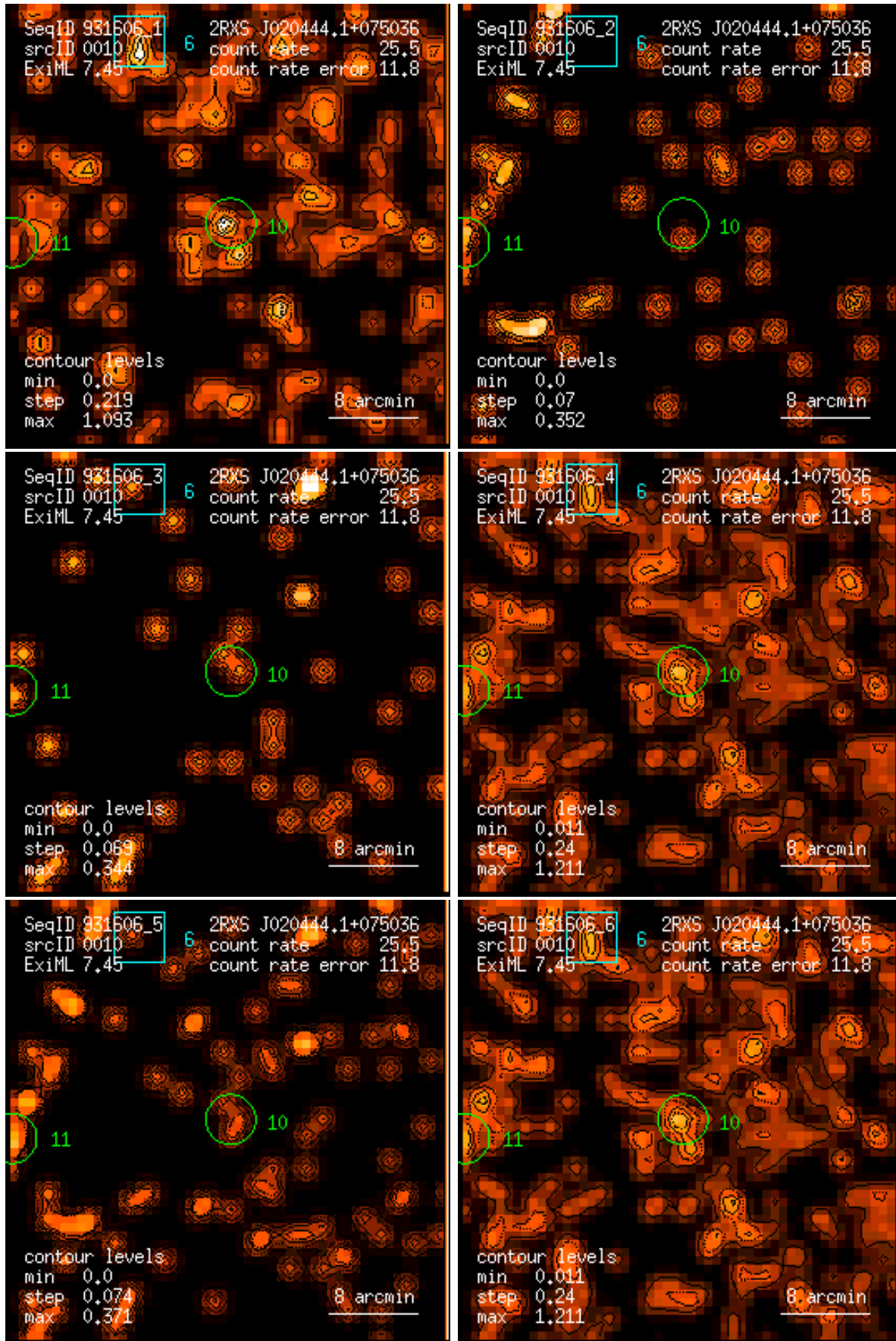
Figure 10: RASS 931606: detection 0010: band rate images, Gaussian filter: (1) PSPC channels 11 – 41, (2) 52 – 90, (3) 91 – 201, (4) 11 – 235, (5) 52 – 201, (6) 11 – 201. Broad band rates in counts/ks. Band rate contour levels in counts/ks/arcmin 2 .
