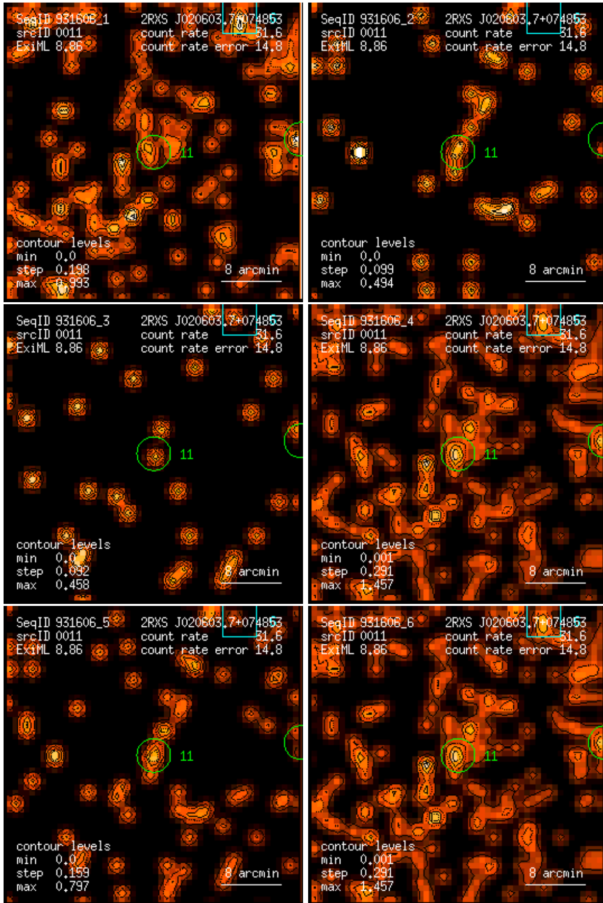
Figure 11: RASS 931606: detection 0011: band rate images, Gaussian filter: (1) PSPC channels 11 – 41, (2) 52 – 90, (3) 91 – 201, (4) 11 – 235, (5) 52 – 201, (6) 11 – 201. Broad band rates in counts/ks. Band rate contour levels in counts/ks/arcmin 2 .
