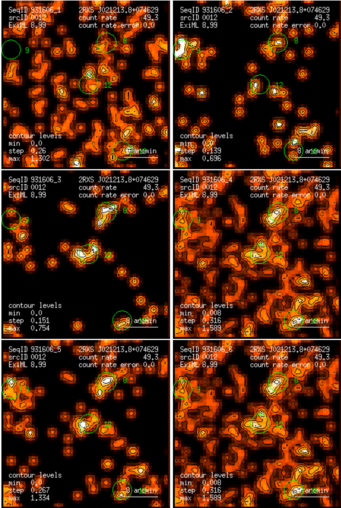
Figure 12: RASS 931606: detection 0012: band rate images, Gaussian filter: (1) PSPC channels 11 – 41, (2) 52 – 90, (3) 91 – 201, (4) 11 – 235, (5) 52 – 201, (6) 11 – 201. Broad band rates in counts/ks. Band rate contour levels in counts/ks/arcmin 2 .
