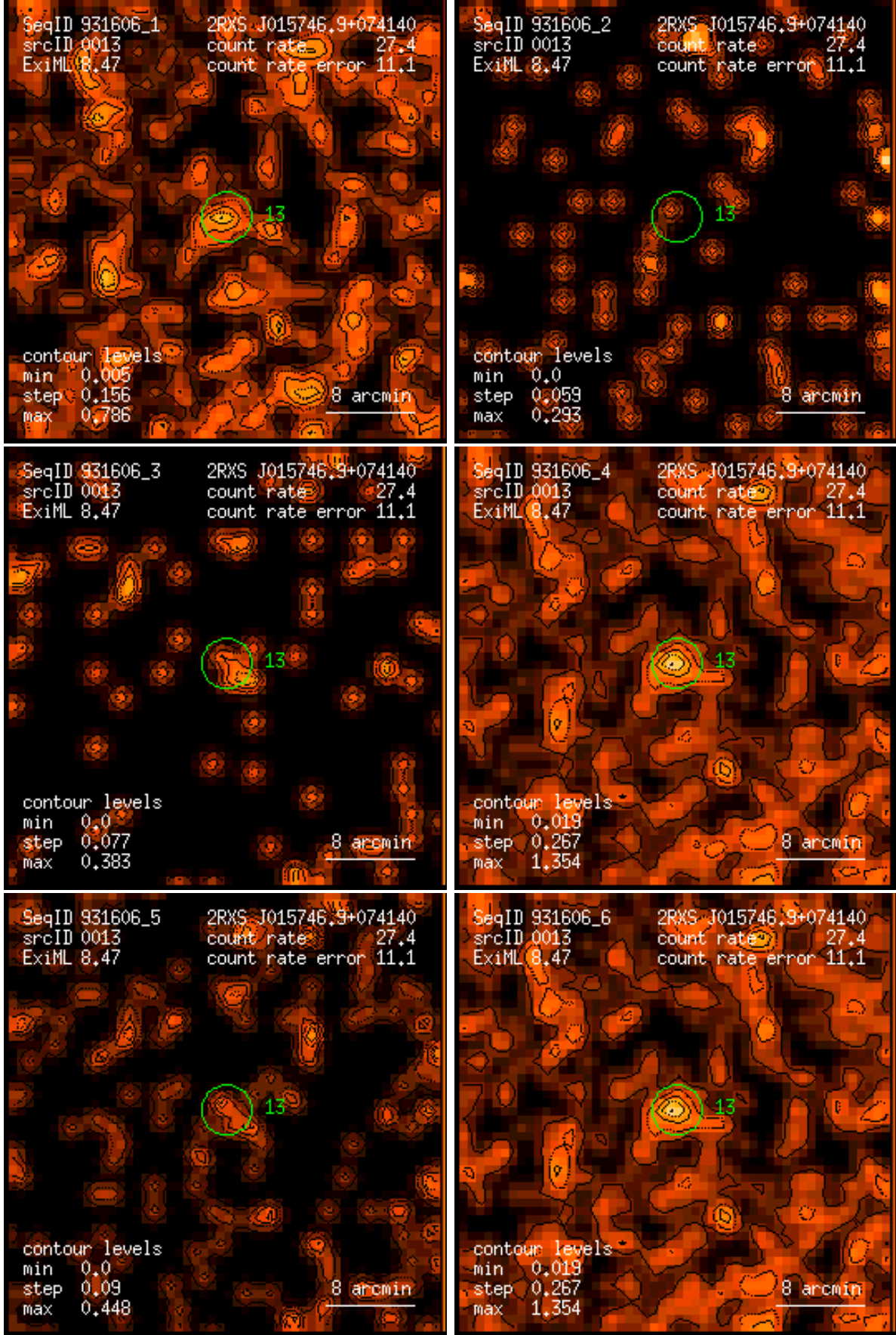
Figure 13: RASS 931606: detection 0013: band rate images, Gaussian filter: (1) PSPC channels 11 – 41, (2) 52 – 90, (3) 91 – 201, (4) 11 – 235, (5) 52 – 201, (6) 11 – 201. Broad band rates in counts/ks. Band rate contour levels in counts/ks/arcmin 2 .
