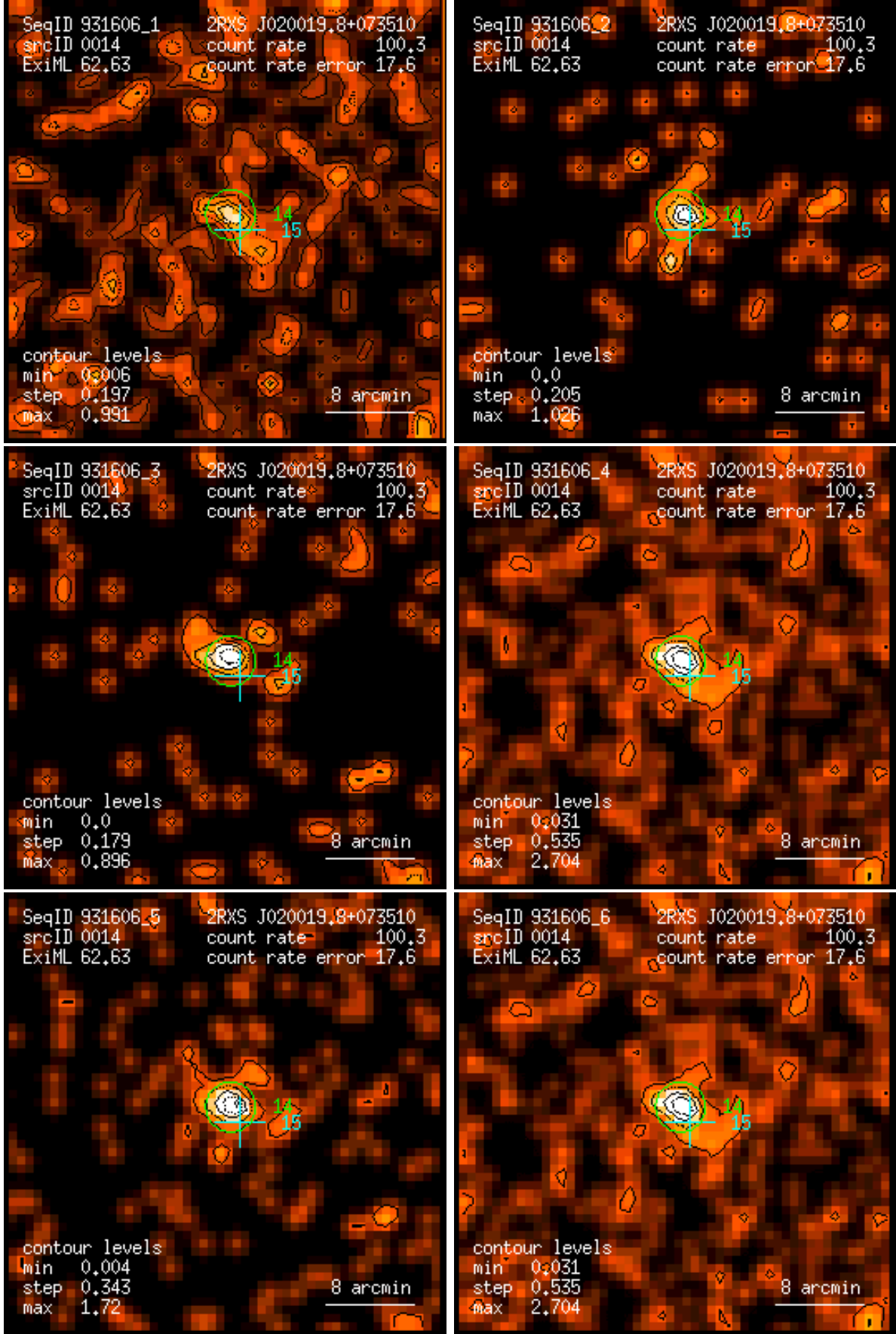
Figure 14: RASS 931606: detection 0014: band rate images, Gaussian filter: (1) PSPC channels 11 – 41, (2) 52 – 90, (3) 91 – 201, (4) 11 – 235, (5) 52 – 201, (6) 11 – 201. Broad band rates in counts/ks. Band rate contour levels in counts/ks/arcmin 2 .
