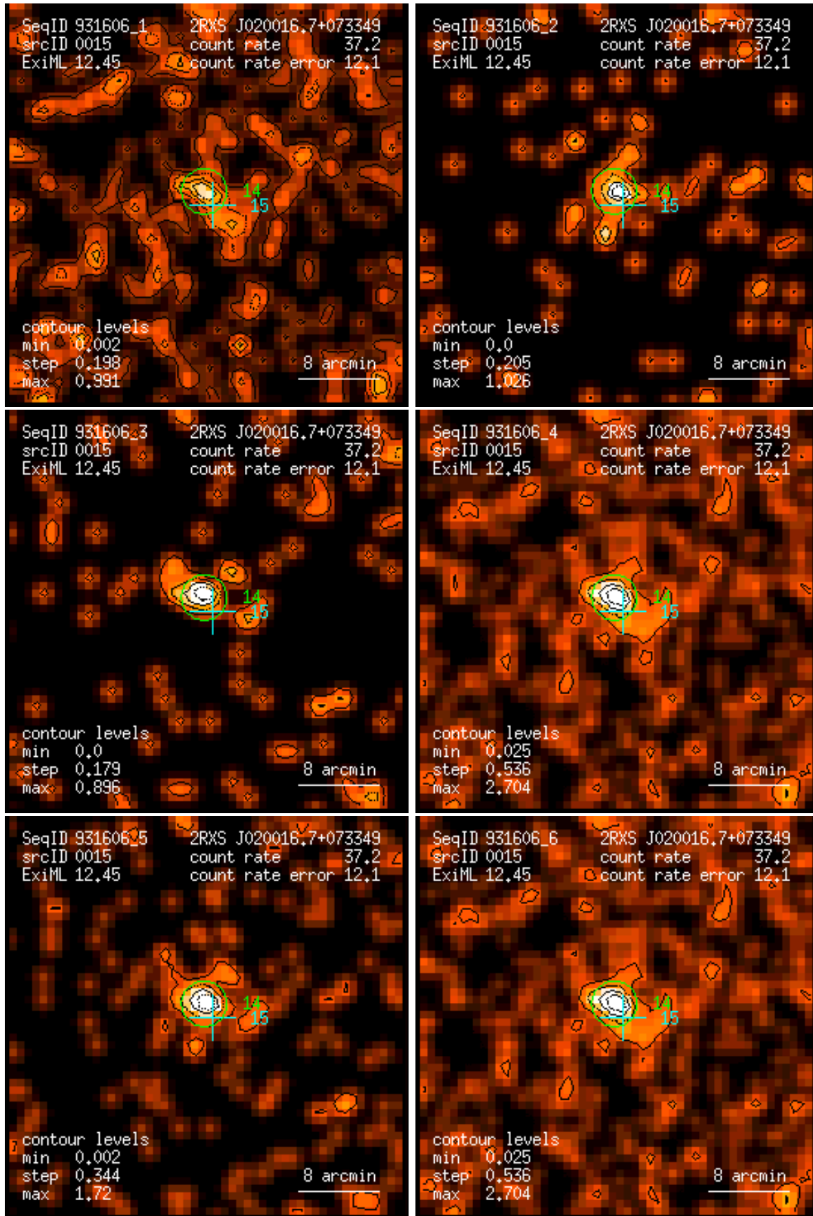
Figure 15: RASS 931606: detection 0015: band rate images, Gaussian filter: (1) PSPC channels 11 – 41, (2) 52 – 90, (3) 91 – 201, (4) 11 – 235, (5) 52 – 201, (6) 11 – 201. Broad band rates in counts/ks. Band rate contour levels in counts/ks/arcmin 2 .
