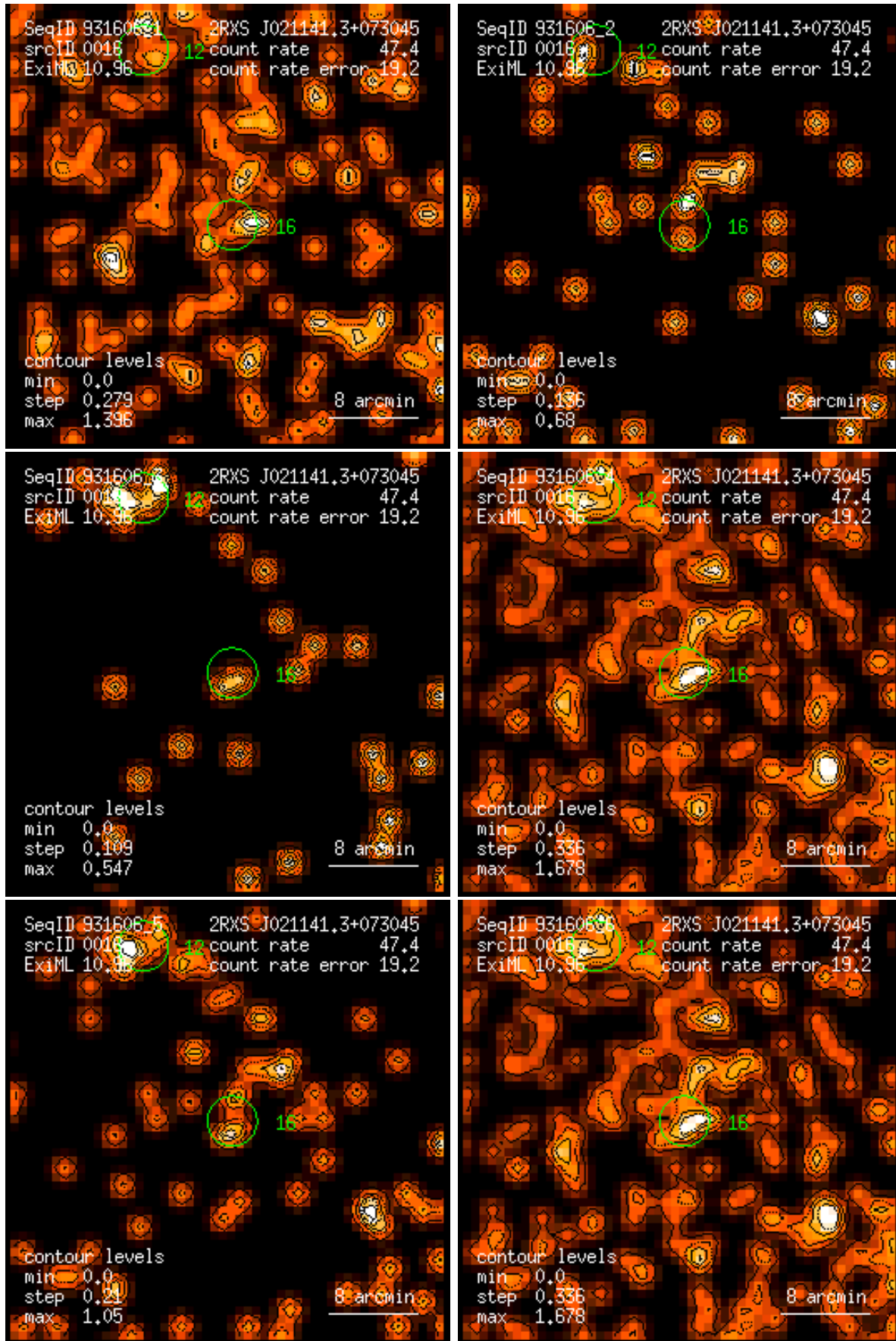
Figure 16: RASS 931606: detection 0016: band rate images, Gaussian filter: (1) PSPC channels 11 – 41, (2) 52 – 90, (3) 91 – 201, (4) 11 – 235, (5) 52 – 201, (6) 11 – 201. Broad band rates in counts/ks. Band rate contour levels in counts/ks/arcmin 2 .
