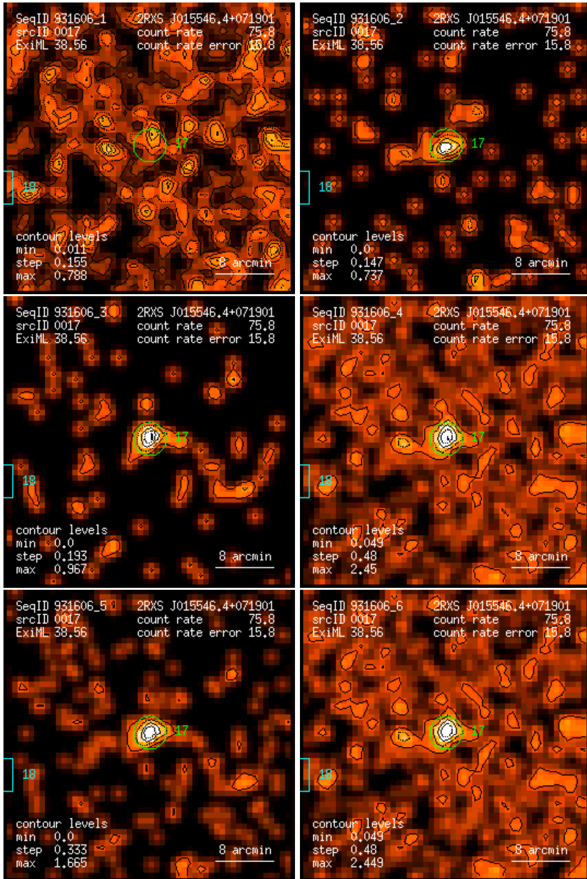
Figure 17: RASS 931606: detection 0017: band rate images, Gaussian filter: (1) PSPC channels 11 – 41, (2) 52 – 90, (3) 91 – 201, (4) 11 – 235, (5) 52 – 201, (6) 11 – 201. Broad band rates in counts/ks. Band rate contour levels in counts/ks/arcmin 2 .
