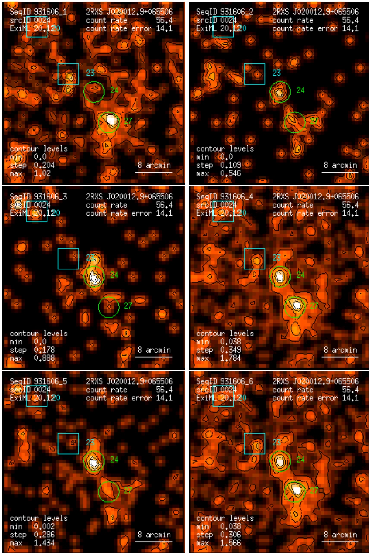
Figure 24: RASS 931606: detection 0024: band rate images, Gaussian filter: (1) PSPC channels 11 – 41, (2) 52 – 90, (3) 91 – 201, (4) 11 – 235, (5) 52 – 201, (6) 11 – 201. Broad band rates in counts/ks. Band rate contour levels in counts/ks/arcmin 2 .
