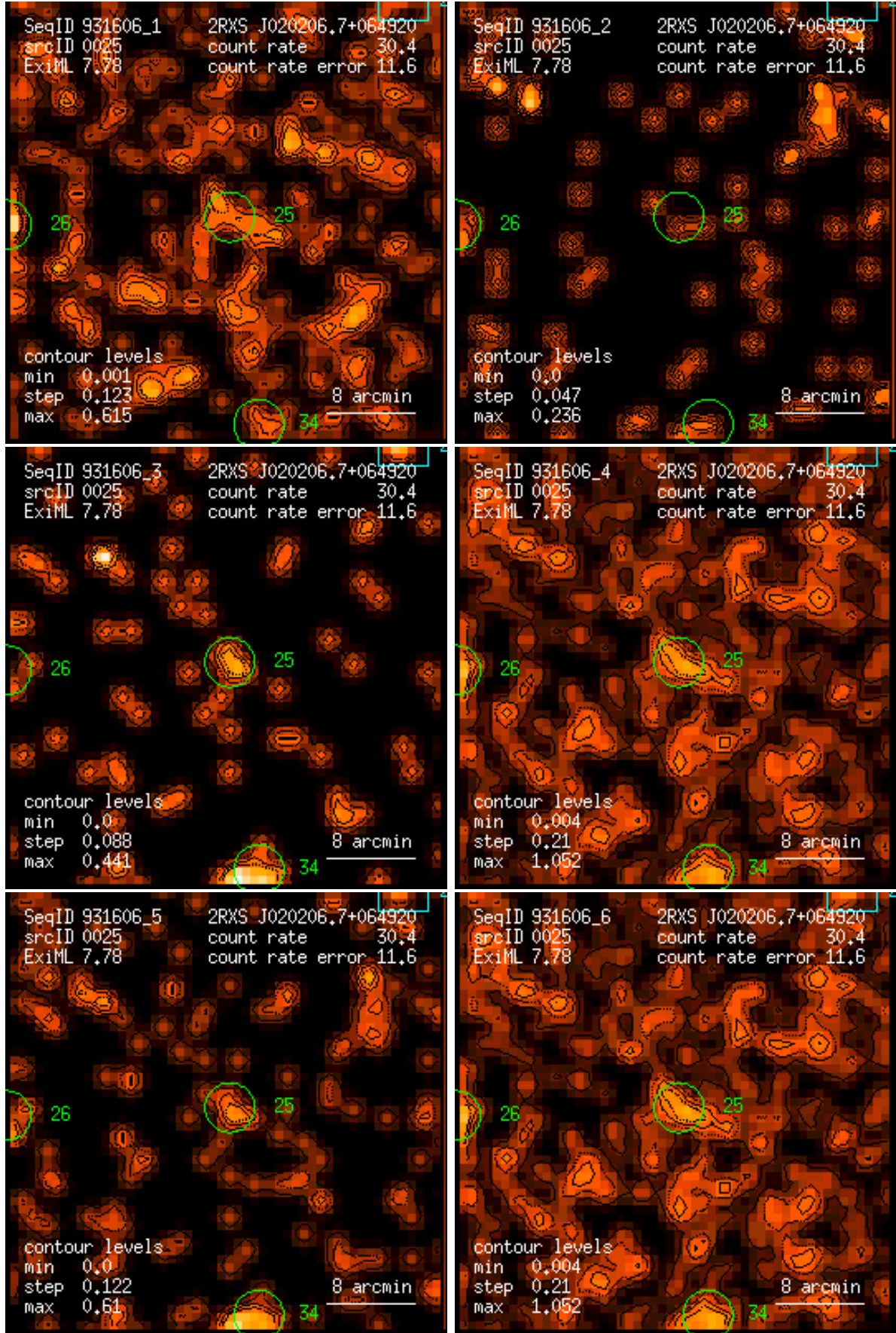
Figure 25: RASS 931606: detection 0025: band rate images, Gaussian filter: (1) PSPC channels 11 – 41, (2) 52 – 90, (3) 91 – 201, (4) 11 – 235, (5) 52 – 201, (6) 11 – 201. Broad band rates in counts/ks. Band rate contour levels in counts/ks/arcmin 2 .
