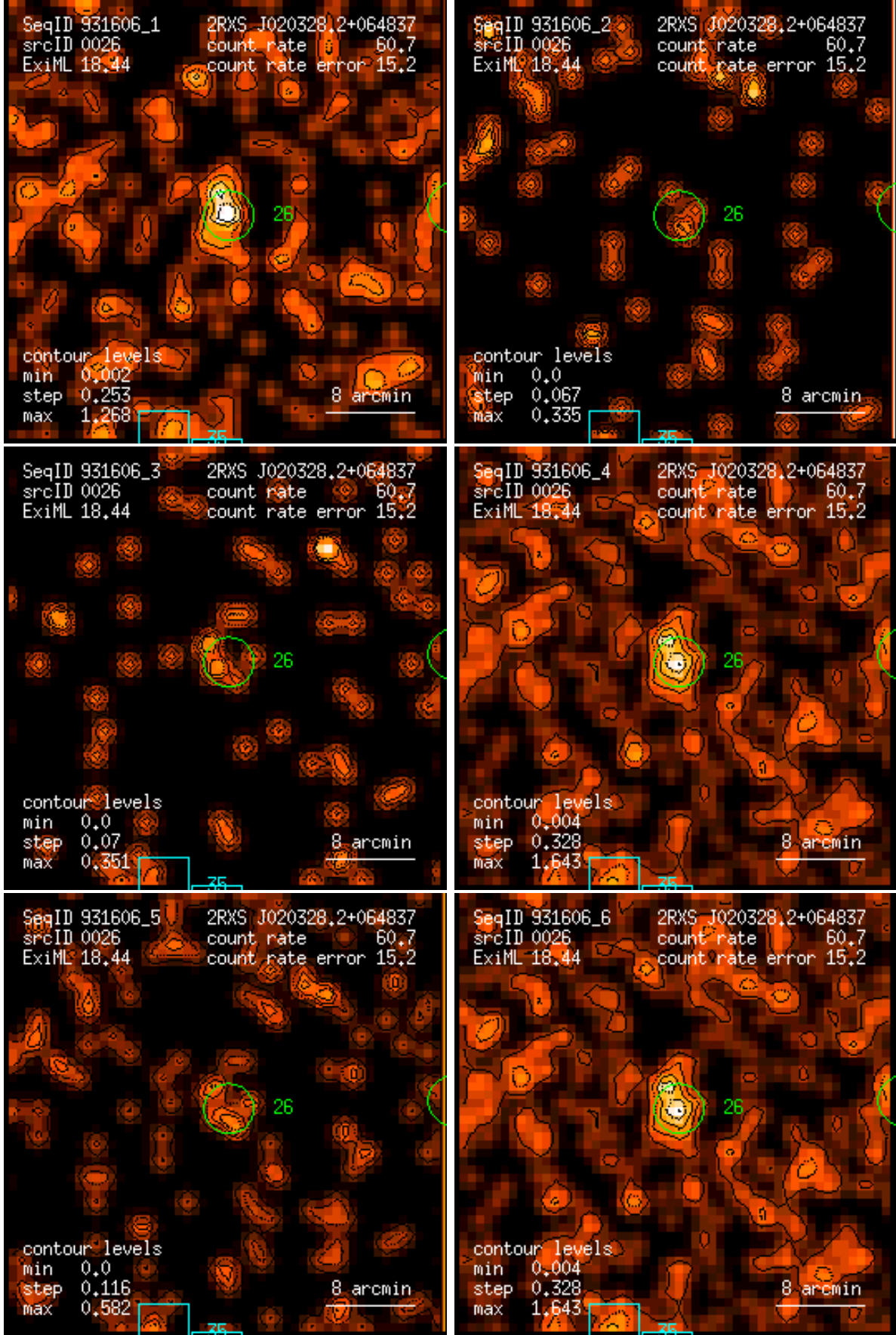
Figure 26: RASS 931606: detection 0026: band rate images, Gaussian filter: (1) PSPC channels 11 – 41, (2) 52 – 90, (3) 91 – 201, (4) 11 – 235, (5) 52 – 201, (6) 11 – 201. Broad band rates in counts/ks. Band rate contour levels in counts/ks/arcmin 2 .
